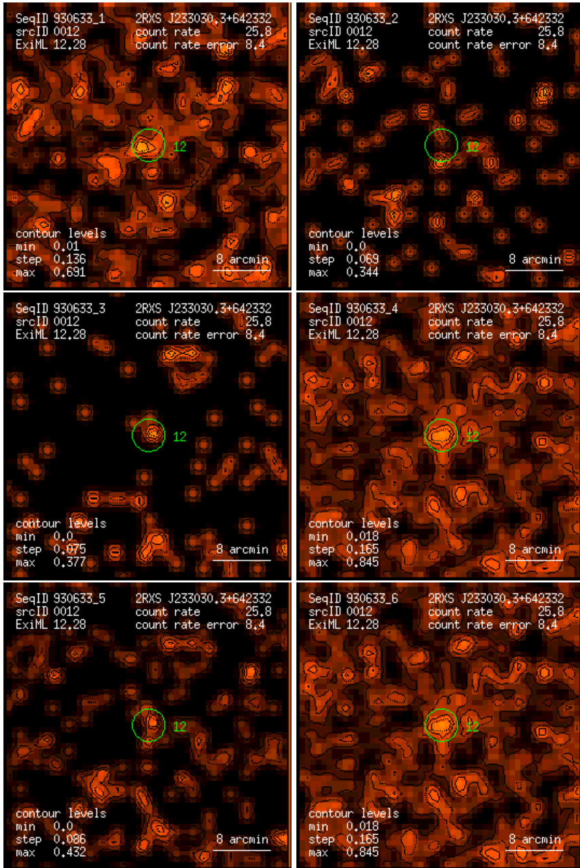
Figure 12: RASS 930633: detection 0012: band rate images, Gaussian filter: (1) PSPC channels 11 – 41, (2) 52 – 90, (3) 91 – 201, (4) 11 – 235, (5) 52 – 201, (6) 11 – 201. Broad band rates in counts/ks. Band rate contour levels in counts/ks/arcmin 2 .
