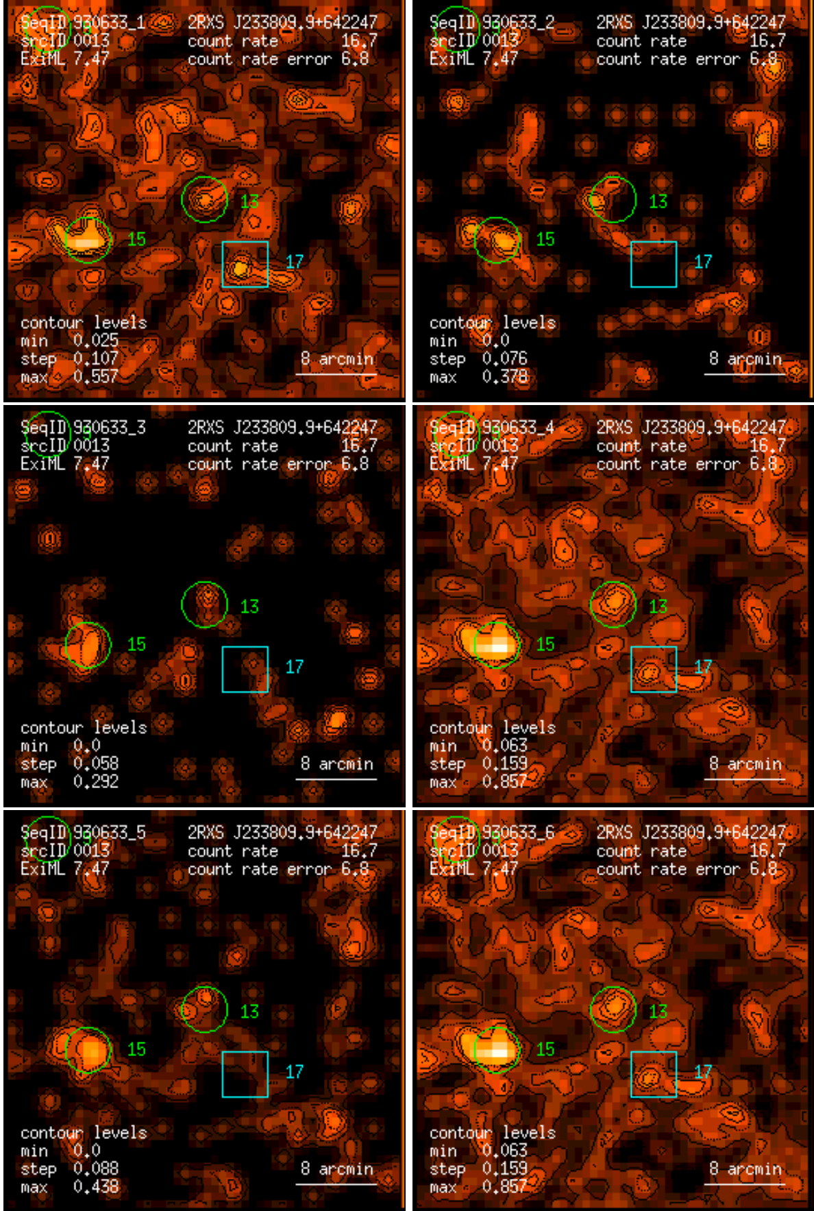
Figure 13: RASS 930633: detection 0013: band rate images, Gaussian filter: (1) PSPC channels 11 – 41, (2) 52 – 90, (3) 91 – 201, (4) 11 – 235, (5) 52 – 201, (6) 11 – 201. Broad band rates in counts/ks. Band rate contour levels in counts/ks/arcmin 2 .
