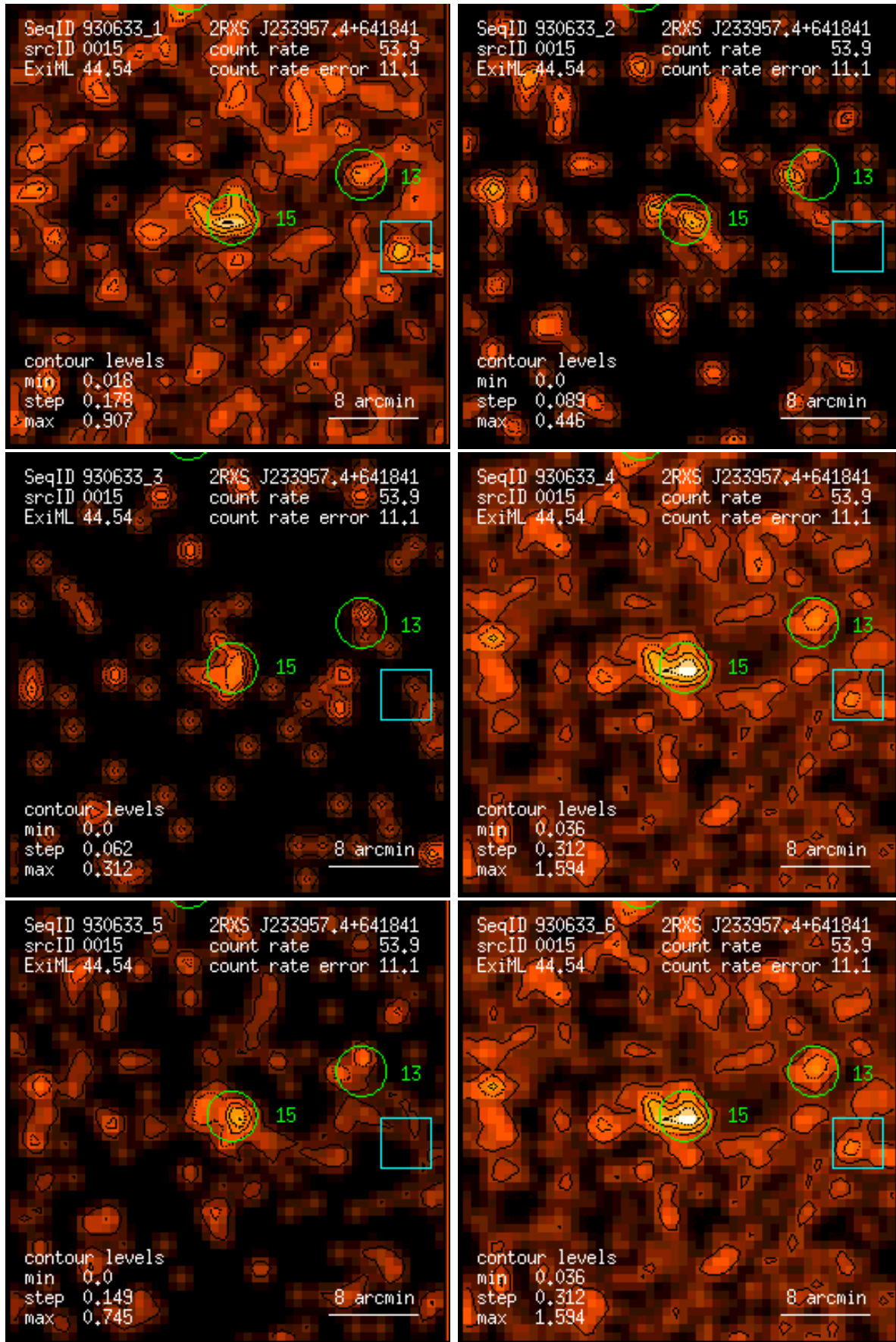
Figure 15: RASS 930633: detection 0015: band rate images, Gaussian filter: (1) PSPC channels 11 – 41, (2) 52 – 90, (3) 91 – 201, (4) 11 – 235, (5) 52 – 201, (6) 11 – 201. Broad band rates in counts/ks. Band rate contour levels in counts/ks/arcmin 2 .
