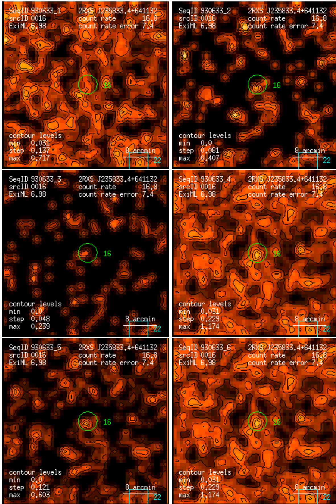
Figure 16: RASS 930633: detection 0016: band rate images, Gaussian filter: (1) PSPC channels 11 – 41, (2) 52 – 90, (3) 91 – 201, (4) 11 – 235, (5) 52 – 201, (6) 11 – 201. Broad band rates in counts/ks. Band rate contour levels in counts/ks/arcmin 2 .
