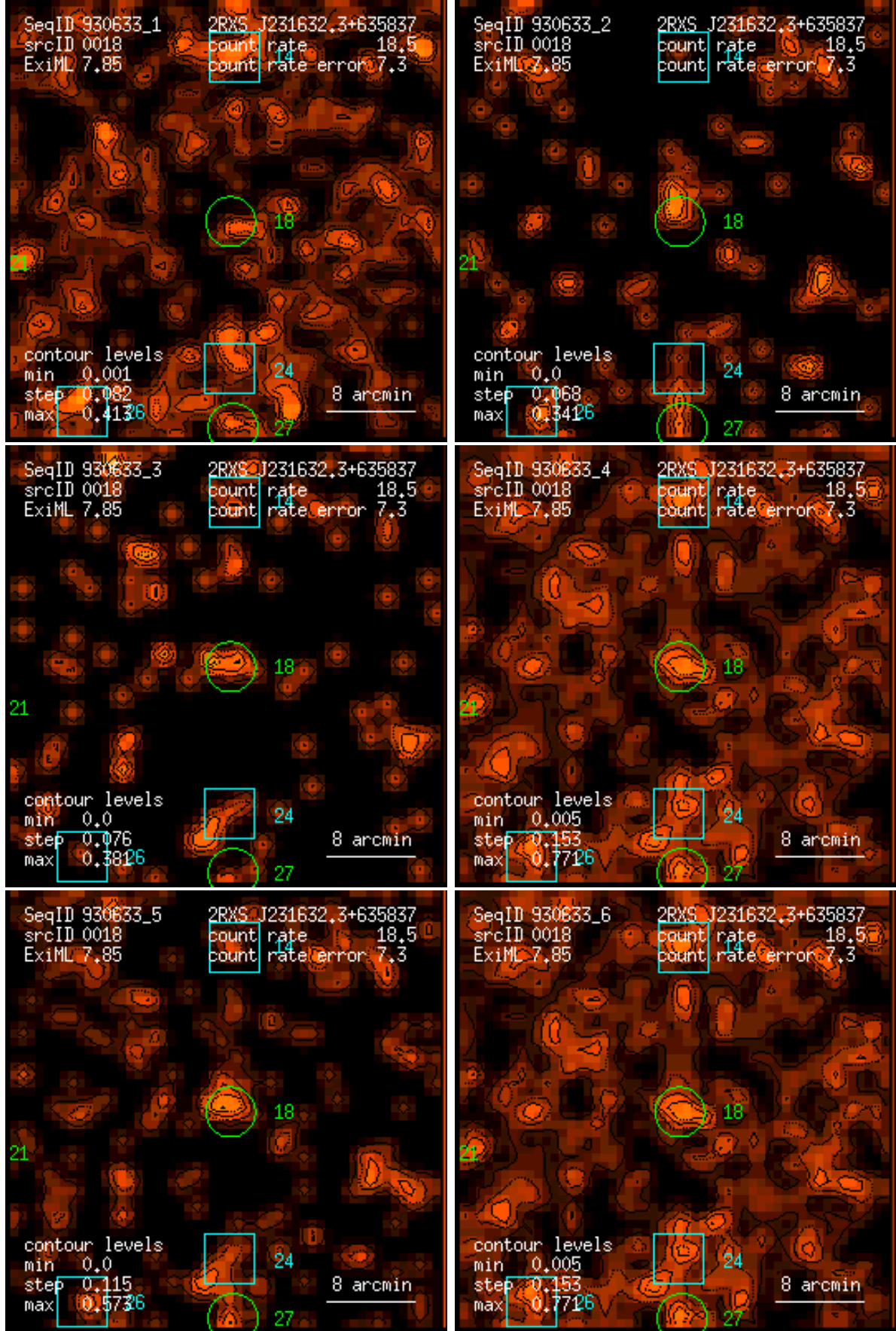
Figure 18: RASS 930633: detection 0018: band rate images, Gaussian filter: (1) PSPC channels 11 – 41, (2) 52 – 90, (3) 91 – 201, (4) 11 – 235, (5) 52 – 201, (6) 11 – 201. Broad band rates in counts/ks. Band rate contour levels in counts/ks/arcmin 2 .
