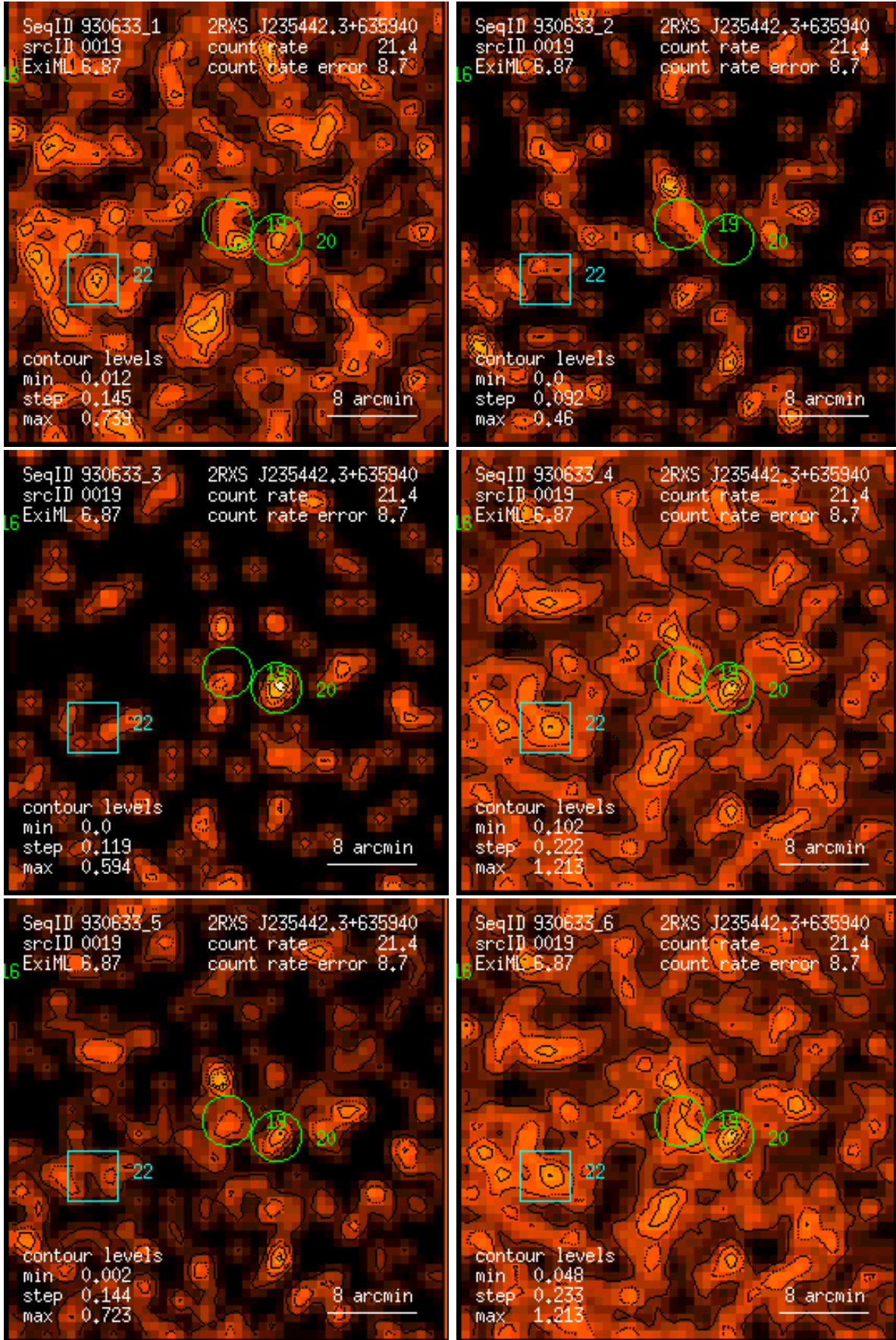
Figure 19: RASS 930633: detection 0019: band rate images, Gaussian filter: (1) PSPC channels 11 – 41, (2) 52 – 90, (3) 91 – 201, (4) 11 – 235, (5) 52 – 201, (6) 11 – 201. Broad band rates in counts/ks. Band rate contour levels in counts/ks/arcmin 2 .
