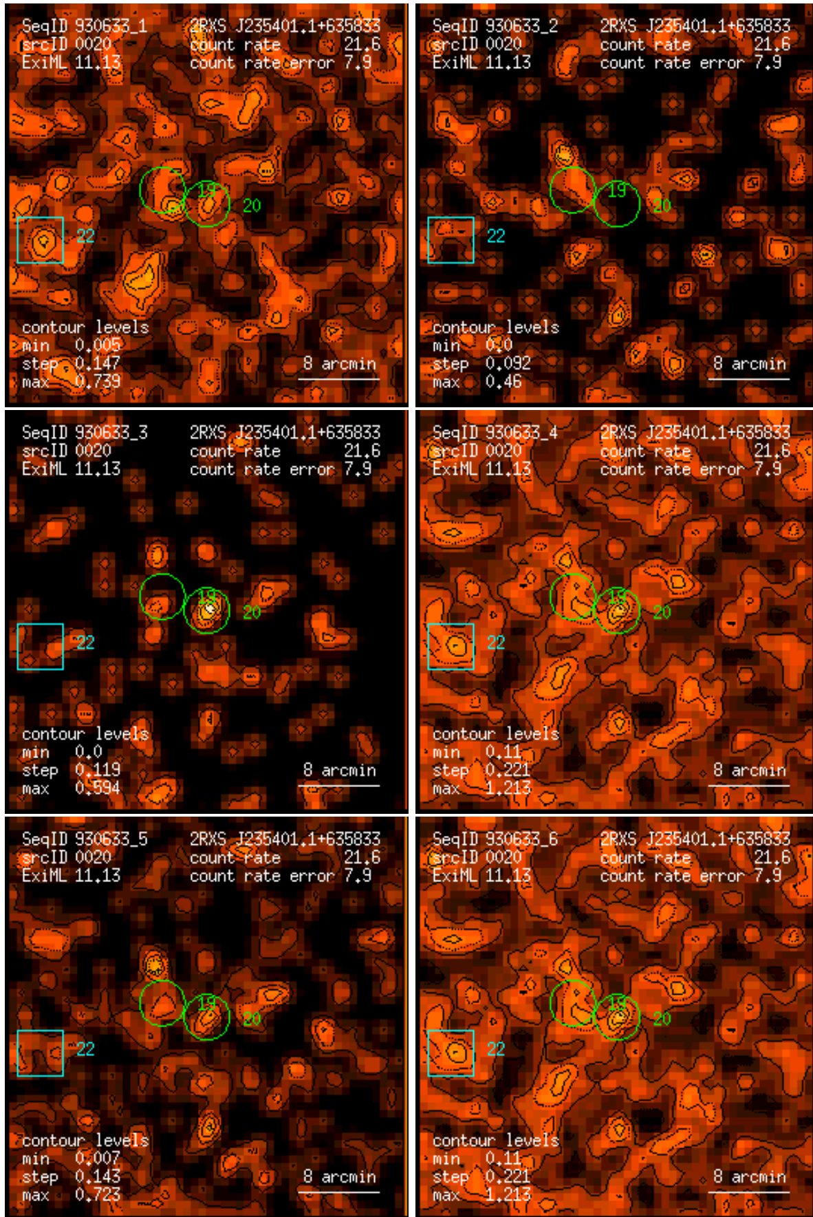
Figure 20: RASS 930633: detection 0020: band rate images, Gaussian filter: (1) PSPC channels 11 – 41, (2) 52 – 90, (3) 91 – 201, (4) 11 – 235, (5) 52 – 201, (6) 11 – 201. Broad band rates in counts/ks. Band rate contour levels in counts/ks/arcmin 2 .
