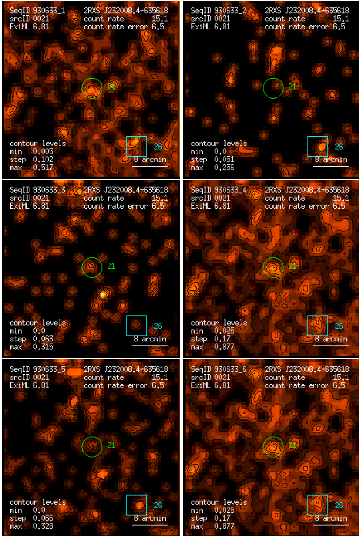
Figure 21: RASS 930633: detection 0021: band rate images, Gaussian filter: (1) PSPC channels 11 – 41, (2) 52 – 90, (3) 91 – 201, (4) 11 – 235, (5) 52 – 201, (6) 11 – 201. Broad band rates in counts/ks. Band rate contour levels in counts/ks/arcmin 2 .
