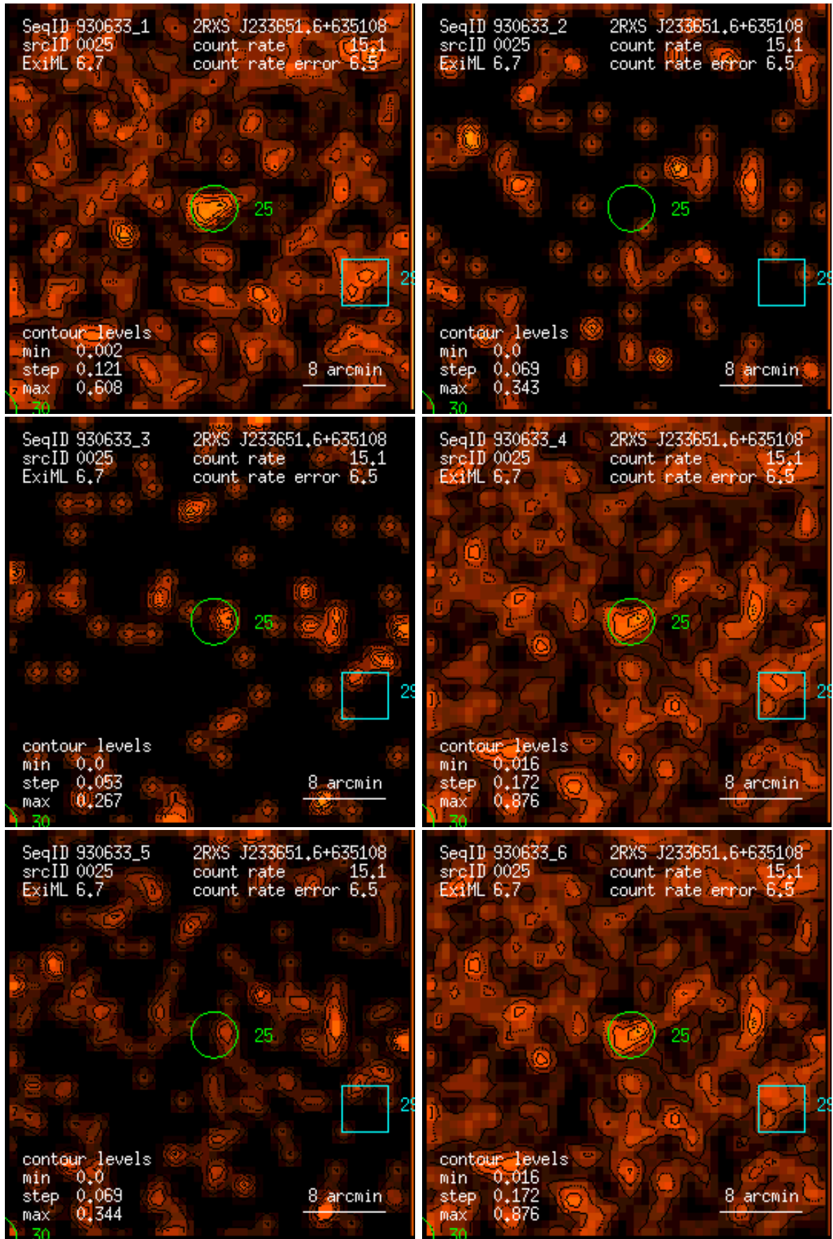
Figure 25: RASS 930633: detection 0025: band rate images, Gaussian filter: (1) PSPC channels 11 – 41, (2) 52 – 90, (3) 91 – 201, (4) 11 – 235, (5) 52 – 201, (6) 11 – 201. Broad band rates in counts/ks. Band rate contour levels in counts/ks/arcmin 2 .
