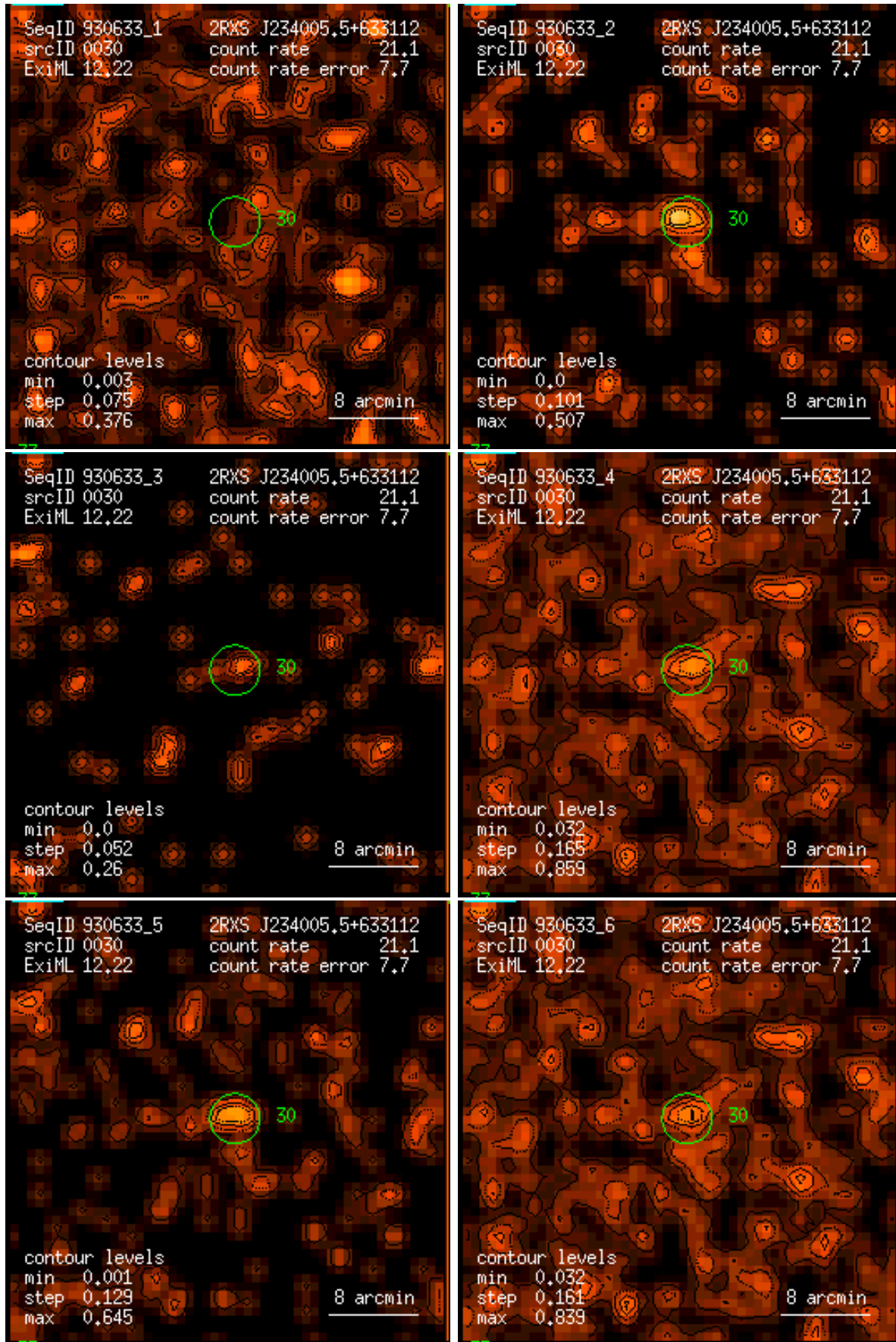
Figure 30: RASS 930633: detection 0030: band rate images, Gaussian filter: (1) PSPC channels 11 – 41, (2) 52 – 90, (3) 91 – 201, (4) 11 – 235, (5) 52 – 201, (6) 11 – 201. Broad band rates in counts/ks. Band rate contour levels in counts/ks/arcmin 2 .
