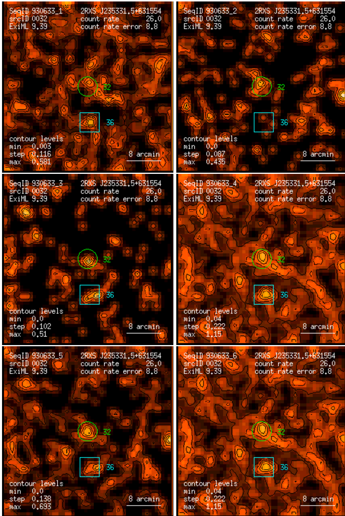
Figure 32: RASS 930633: detection 0032: band rate images, Gaussian filter: (1) PSPC channels 11 – 41, (2) 52 – 90, (3) 91 – 201, (4) 11 – 235, (5) 52 – 201, (6) 11 – 201. Broad band rates in counts/ks. Band rate contour levels in counts/ks/arcmin 2 .
