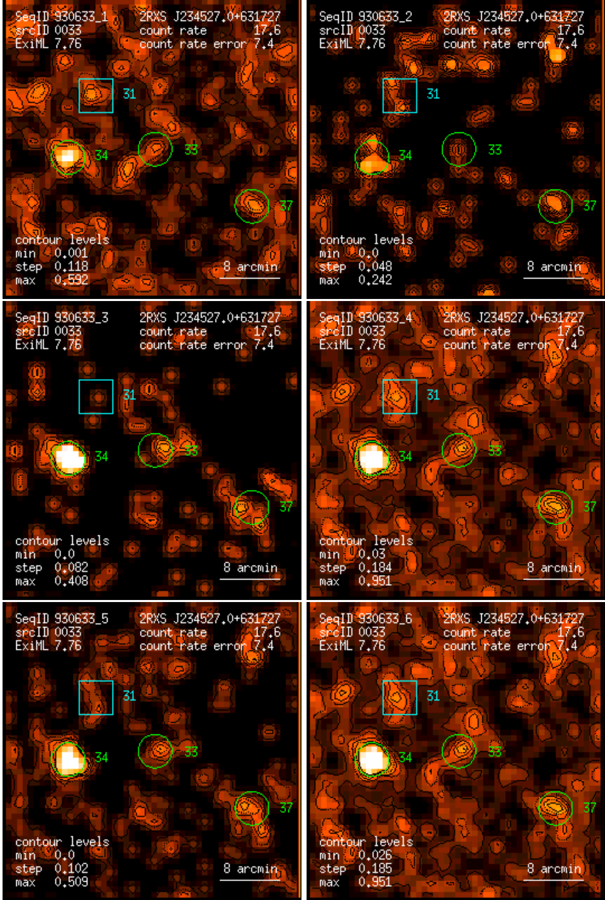
Figure 33: RASS 930633: detection 0033: band rate images, Gaussian filter: (1) PSPC channels 11 – 41, (2) 52 – 90, (3) 91 – 201, (4) 11 – 235, (5) 52 – 201, (6) 11 – 201. Broad band rates in counts/ks. Band rate contour levels in counts/ks/arcmin 2 .
