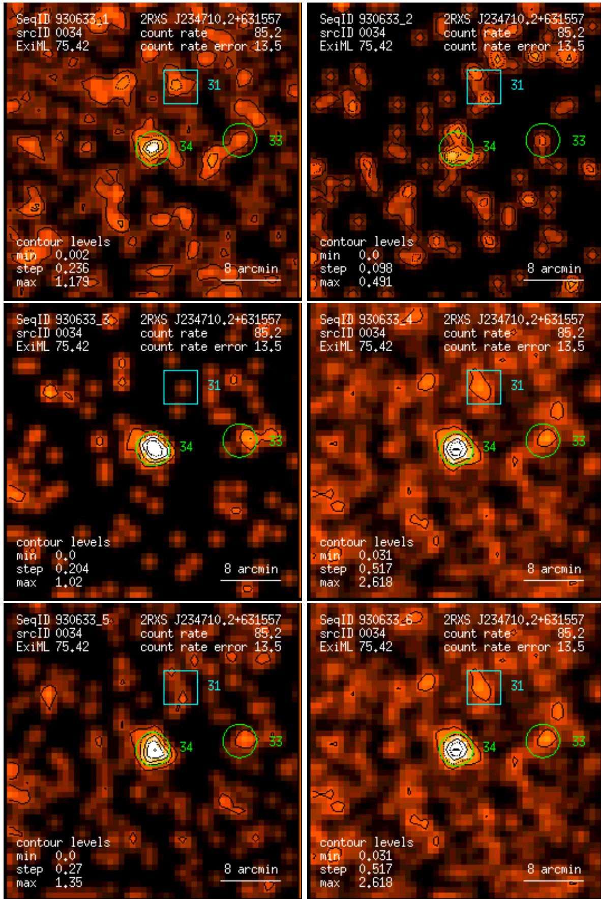
Figure 34: RASS 930633: detection 0034: band rate images, Gaussian filter: (1) PSPC channels 11 – 41, (2) 52 – 90, (3) 91 – 201, (4) 11 – 235, (5) 52 – 201, (6) 11 – 201. Broad band rates in counts/ks. Band rate contour levels in counts/ks/arcmin 2 .
