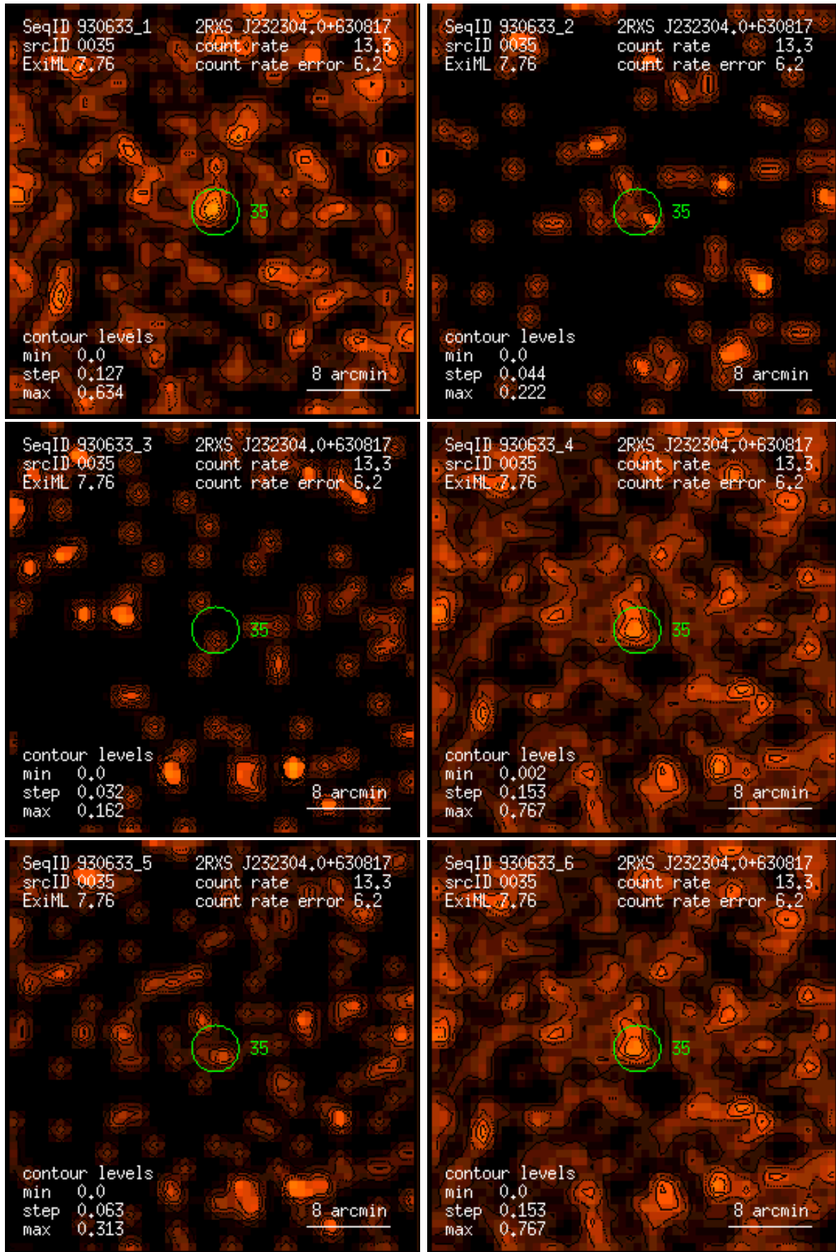
Figure 35: RASS 930633: detection 0035: band rate images, Gaussian filter: (1) PSPC channels 11 – 41, (2) 52 – 90, (3) 91 – 201, (4) 11 – 235, (5) 52 – 201, (6) 11 – 201. Broad band rates in counts/ks. Band rate contour levels in counts/ks/arcmin 2 .
