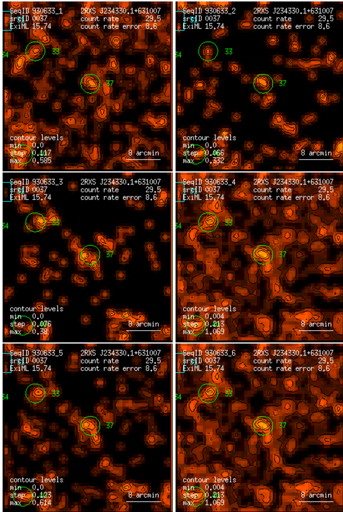
Figure 37: RASS 930633: detection 0037: band rate images, Gaussian filter: (1) PSPC channels 11 – 41, (2) 52 – 90, (3) 91 – 201, (4) 11 – 235, (5) 52 – 201, (6) 11 – 201. Broad band rates in counts/ks. Band rate contour levels in counts/ks/arcmin 2 .
