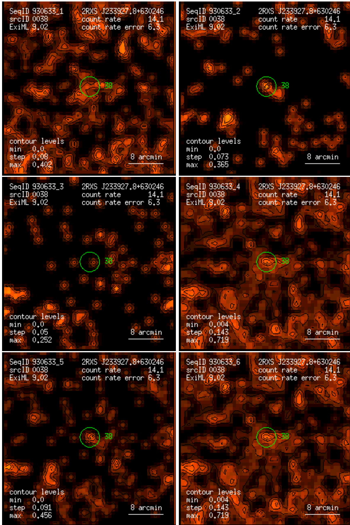
Figure 38: RASS 930633: detection 0038: band rate images, Gaussian filter: (1) PSPC channels 11 – 41, (2) 52 – 90, (3) 91 – 201, (4) 11 – 235, (5) 52 – 201, (6) 11 – 201. Broad band rates in counts/ks. Band rate contour levels in counts/ks/arcmin 2 .
