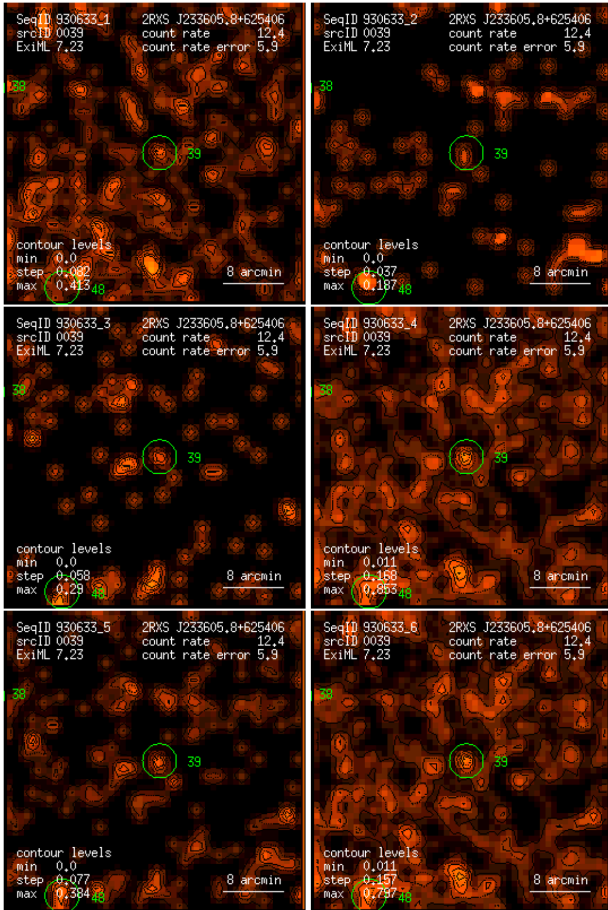
Figure 39: RASS 930633: detection 0039: band rate images, Gaussian filter: (1) PSPC channels 11 – 41, (2) 52 – 90, (3) 91 – 201, (4) 11 – 235, (5) 52 – 201, (6) 11 – 201. Broad band rates in counts/ks. Band rate contour levels in counts/ks/arcmin 2 .
