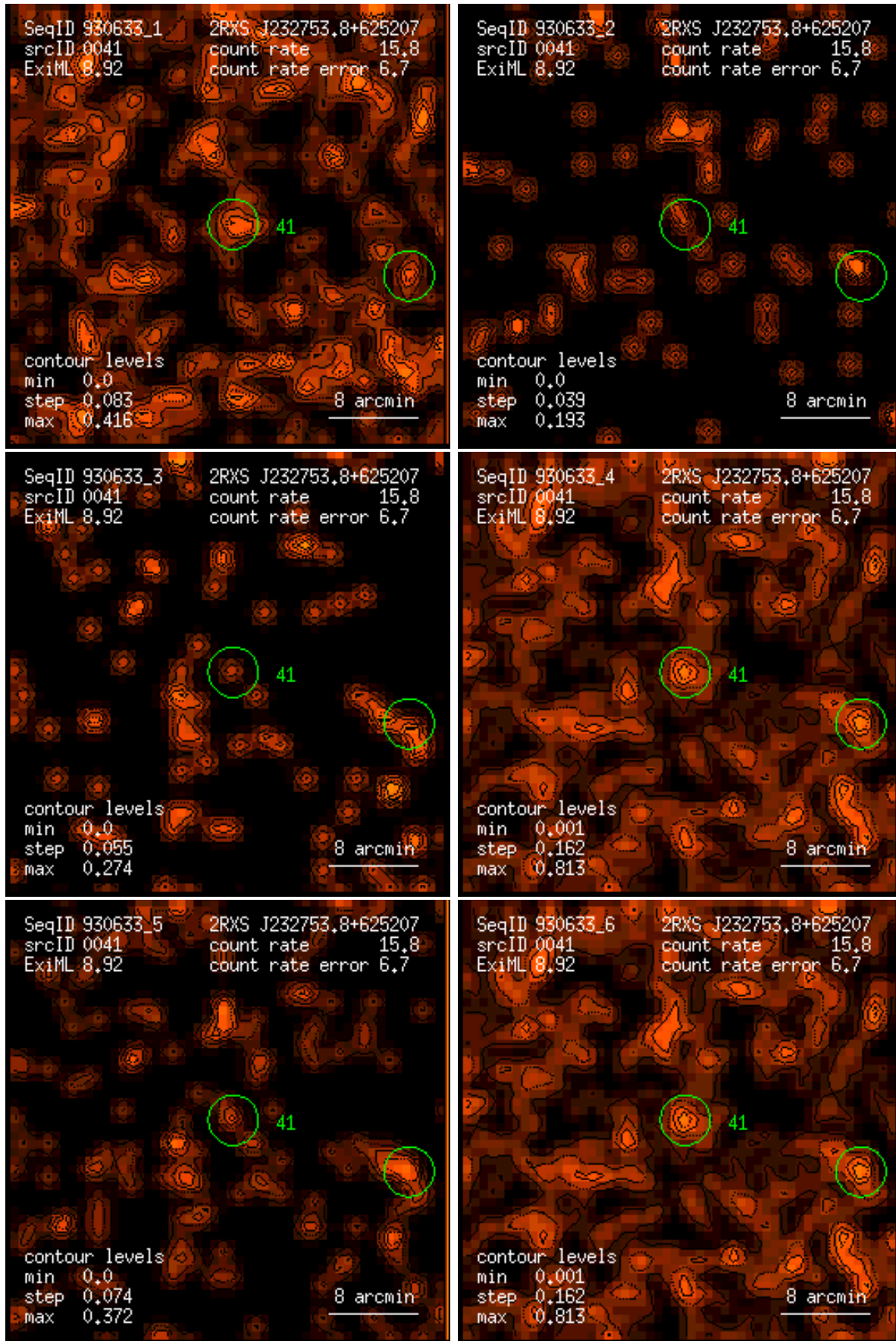
Figure 41: RASS 930633: detection 0041: band rate images, Gaussian filter: (1) PSPC channels 11 – 41, (2) 52 – 90, (3) 91 – 201, (4) 11 – 235, (5) 52 – 201, (6) 11 – 201. Broad band rates in counts/ks. Band rate contour levels in counts/ks/arcmin 2 .
