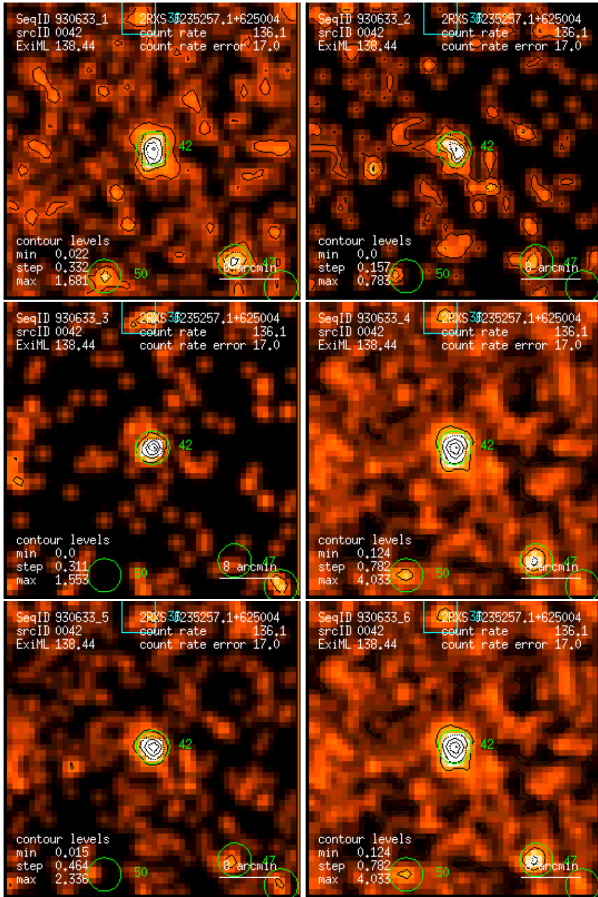
Figure 42: RASS 930633: detection 0042: band rate images, Gaussian filter: (1) PSPC channels 11 – 41, (2) 52 – 90, (3) 91 – 201, (4) 11 – 235, (5) 52 – 201, (6) 11 – 201. Broad band rates in counts/ks. Band rate contour levels in counts/ks/arcmin 2 .
