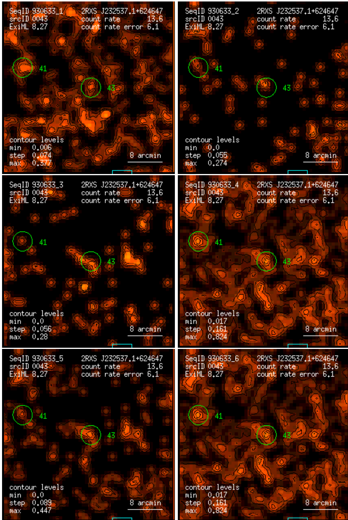
Figure 43: RASS 930633: detection 0043: band rate images, Gaussian filter: (1) PSPC channels 11 – 41, (2) 52 – 90, (3) 91 – 201, (4) 11 – 235, (5) 52 – 201, (6) 11 – 201. Broad band rates in counts/ks. Band rate contour levels in counts/ks/arcmin 2 .
