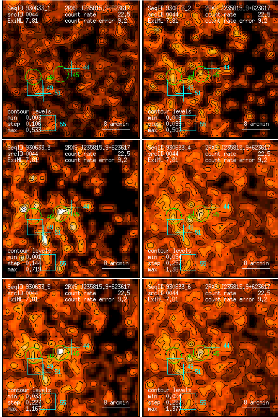
Figure 44: RASS 930633: detection 0044: band rate images, Gaussian filter: (1) PSPC channels 11 – 41, (2) 52 – 90, (3) 91 – 201, (4) 11 – 235, (5) 52 – 201, (6) 11 – 201. Broad band rates in counts/ks. Band rate contour levels in counts/ks/arcmin 2 .
