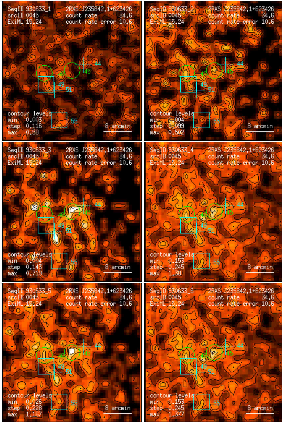
Figure 45: RASS 930633: detection 0045: band rate images, Gaussian filter: (1) PSPC channels 11 – 41, (2) 52 – 90, (3) 91 – 201, (4) 11 – 235, (5) 52 – 201, (6) 11 – 201. Broad band rates in counts/ks. Band rate contour levels in counts/ks/arcmin 2 .
