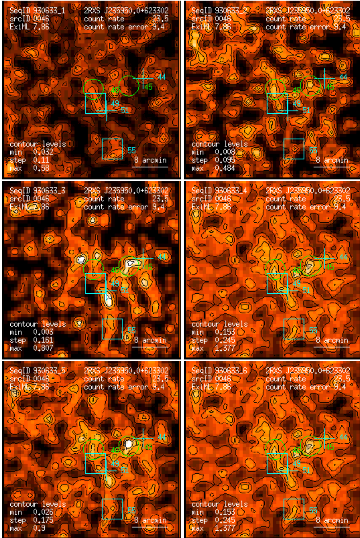
Figure 46: RASS 930633: detection 0046: band rate images, Gaussian filter: (1) PSPC channels 11 – 41, (2) 52 – 90, (3) 91 – 201, (4) 11 – 235, (5) 52 – 201, (6) 11 – 201. Broad band rates in counts/ks. Band rate contour levels in counts/ks/arcmin 2 .
