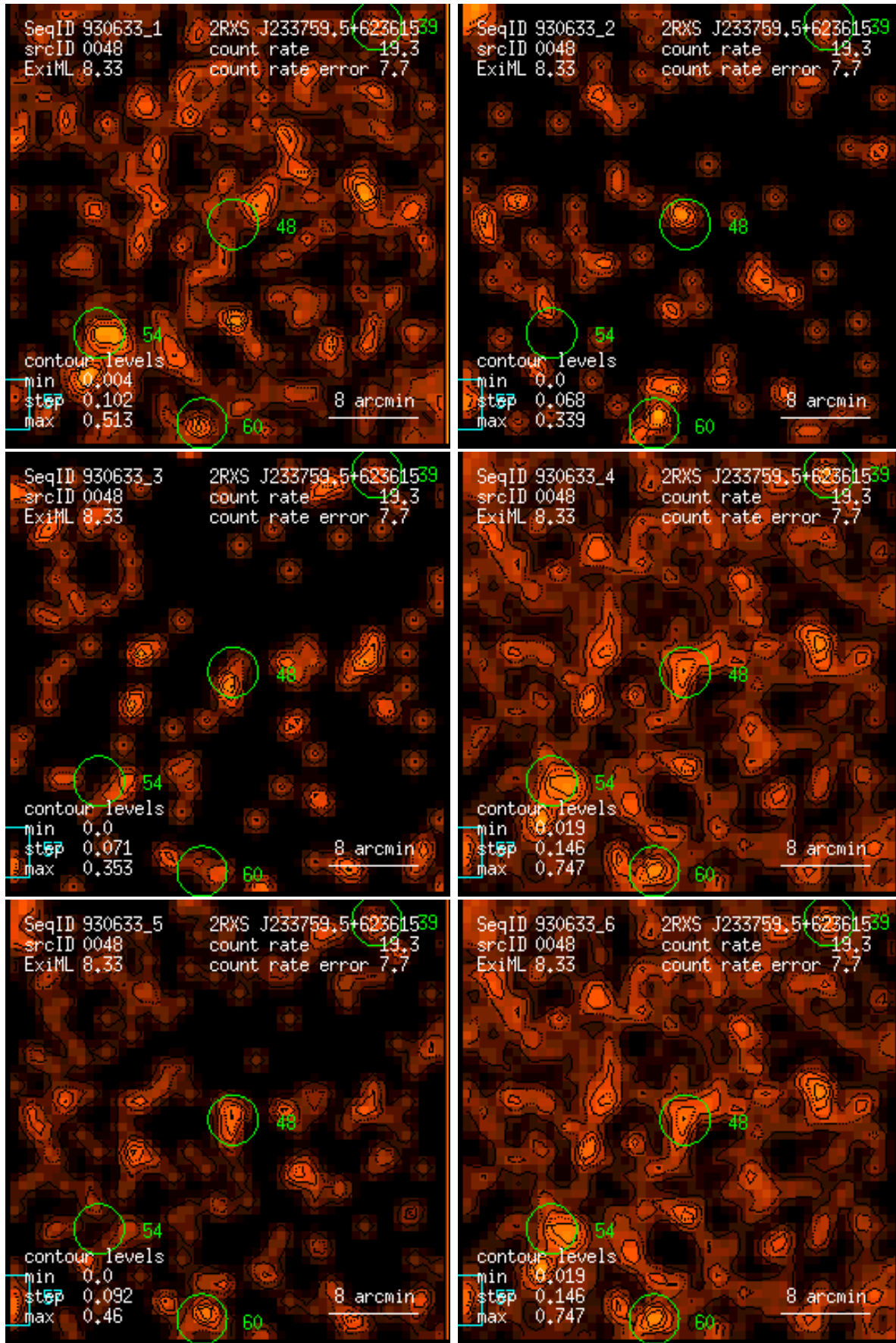
Figure 48: RASS 930633: detection 0048: band rate images, Gaussian filter: (1) PSPC channels 11 – 41, (2) 52 – 90, (3) 91 – 201, (4) 11 – 235, (5) 52 – 201, (6) 11 – 201. Broad band rates in counts/ks. Band rate contour levels in counts/ks/arcmin 2 .
