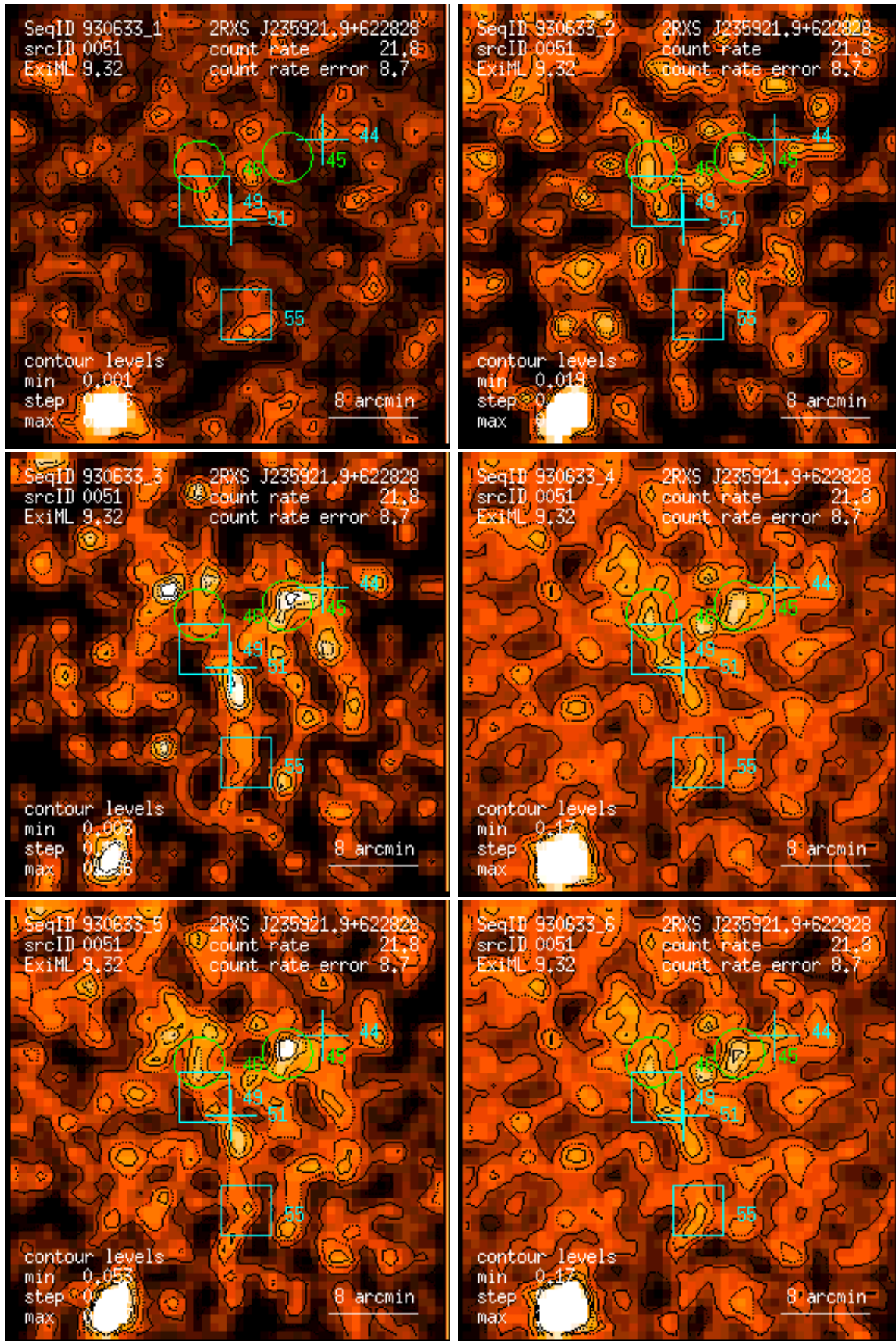
Figure 51: RASS 930633: detection 0051: band rate images, Gaussian filter: (1) PSPC channels 11 – 41, (2) 52 – 90, (3) 91 – 201, (4) 11 – 235, (5) 52 – 201, (6) 11 – 201. Broad band rates in counts/ks. Band rate contour levels in counts/ks/arcmin 2 .
