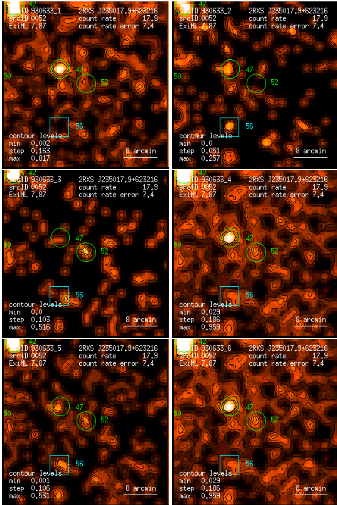
Figure 52: RASS 930633: detection 0052: band rate images, Gaussian filter: (1) PSPC channels 11 – 41, (2) 52 – 90, (3) 91 – 201, (4) 11 – 235, (5) 52 – 201, (6) 11 – 201. Broad band rates in counts/ks. Band rate contour levels in counts/ks/arcmin 2 .
