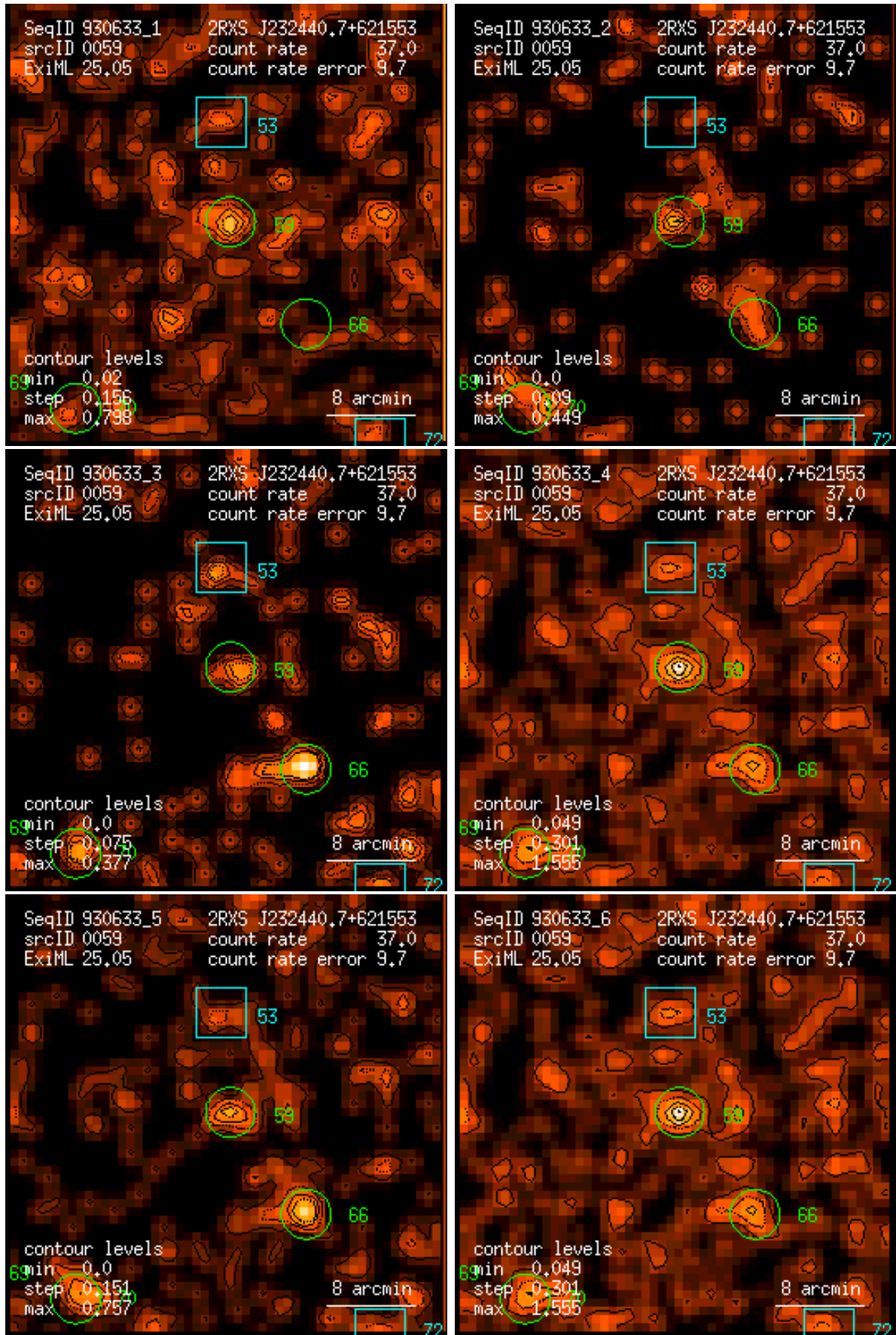
Figure 59: RASS 930633: detection 0059: band rate images, Gaussian filter: (1) PSPC channels 11 – 41, (2) 52 – 90, (3) 91 – 201, (4) 11 – 235, (5) 52 – 201, (6) 11 – 201. Broad band rates in counts/ks. Band rate contour levels in counts/ks/arcmin 2 .
