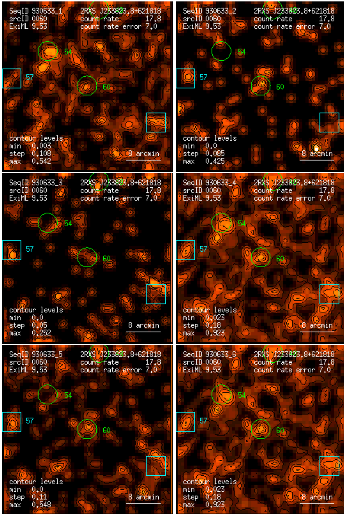
Figure 60: RASS 930633: detection 0060: band rate images, Gaussian filter: (1) PSPC channels 11 – 41, (2) 52 – 90, (3) 91 – 201, (4) 11 – 235, (5) 52 – 201, (6) 11 – 201. Broad band rates in counts/ks. Band rate contour levels in counts/ks/arcmin 2 .
