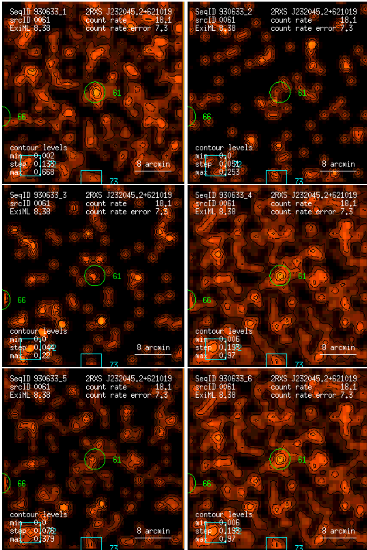
Figure 61: RASS 930633: detection 0061: band rate images, Gaussian filter: (1) PSPC channels 11 – 41, (2) 52 – 90, (3) 91 – 201, (4) 11 – 235, (5) 52 – 201, (6) 11 – 201. Broad band rates in counts/ks. Band rate contour levels in counts/ks/arcmin 2 .
