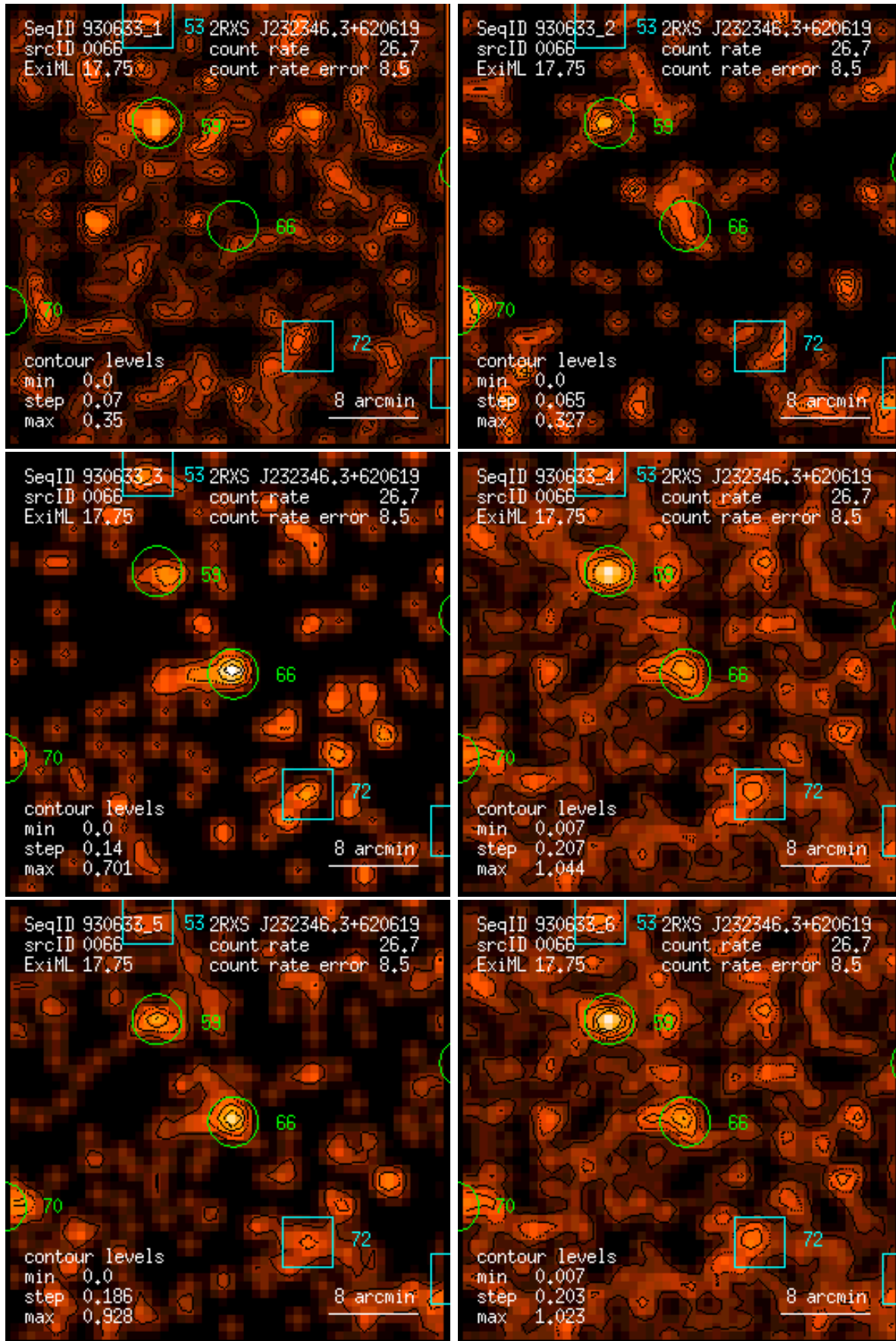
Figure 66: RASS 930633: detection 0066: band rate images, Gaussian filter: (1) PSPC channels 11 – 41, (2) 52 – 90, (3) 91 – 201, (4) 11 – 235, (5) 52 – 201, (6) 11 – 201. Broad band rates in counts/ks. Band rate contour levels in counts/ks/arcmin 2 .
