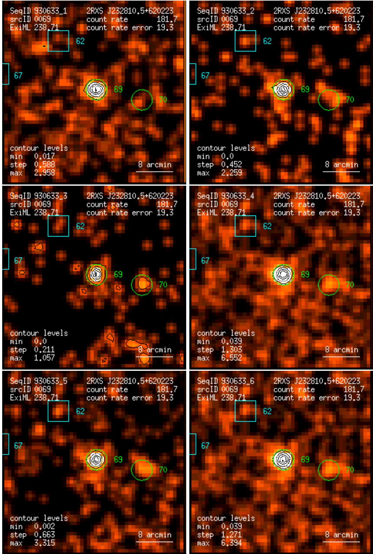
Figure 69: RASS 930633: detection 0069: band rate images, Gaussian filter: (1) PSPC channels 11 – 41, (2) 52 – 90, (3) 91 – 201, (4) 11 – 235, (5) 52 – 201, (6) 11 – 201. Broad band rates in counts/ks. Band rate contour levels in counts/ks/arcmin 2 .
