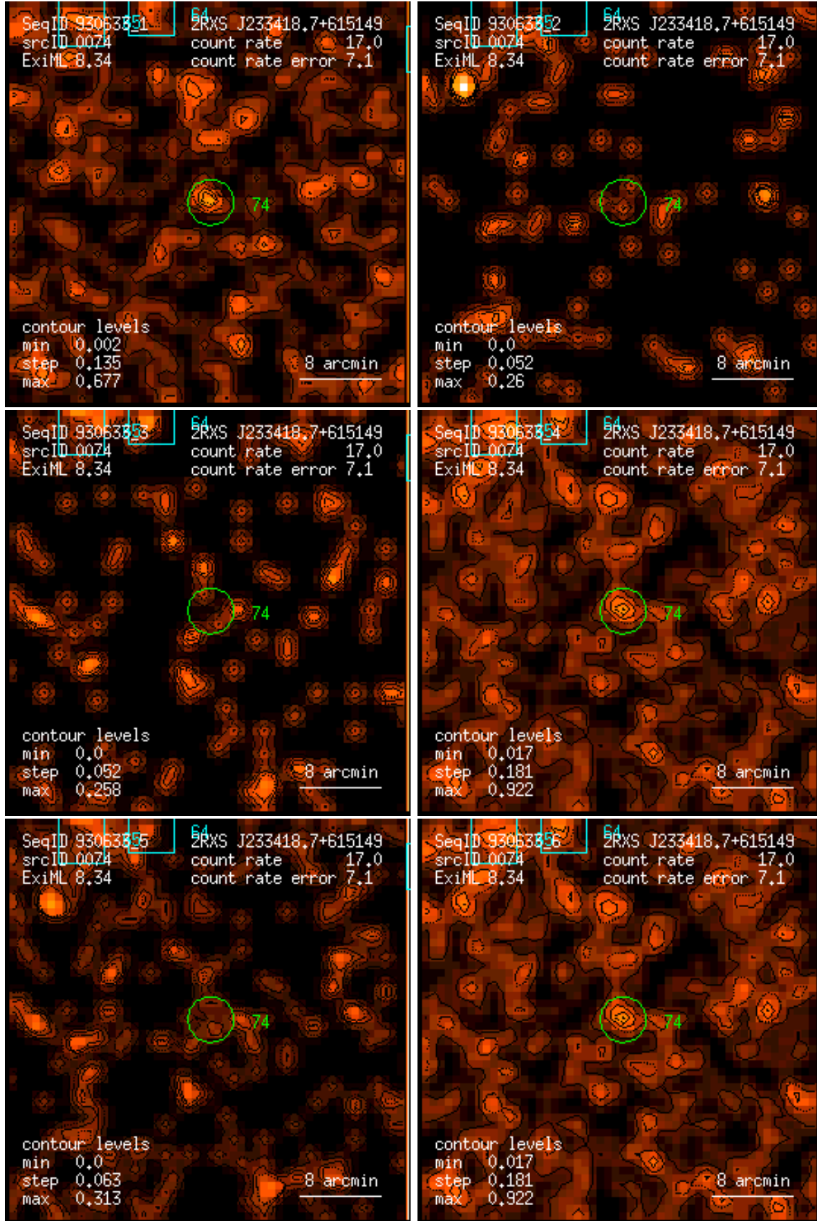
Figure 74: RASS 930633: detection 0074: band rate images, Gaussian filter: (1) PSPC channels 11 – 41, (2) 52 – 90, (3) 91 – 201, (4) 11 – 235, (5) 52 – 201, (6) 11 – 201. Broad band rates in counts/ks. Band rate contour levels in counts/ks/arcmin 2 .
