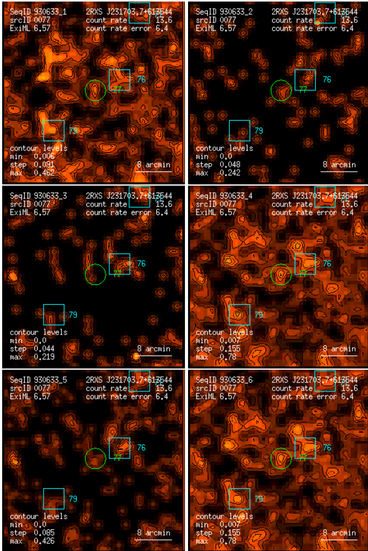
Figure 77: RASS 930633: detection 0077: band rate images, Gaussian filter: (1) PSPC channels 11 – 41, (2) 52 – 90, (3) 91 – 201, (4) 11 – 235, (5) 52 – 201, (6) 11 – 201. Broad band rates in counts/ks. Band rate contour levels in counts/ks/arcmin 2 .
