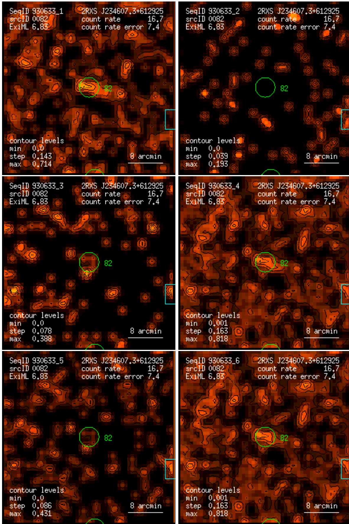
Figure 82: RASS 930633: detection 0082: band rate images, Gaussian filter: (1) PSPC channels 11 – 41, (2) 52 – 90, (3) 91 – 201, (4) 11 – 235, (5) 52 – 201, (6) 11 – 201. Broad band rates in counts/ks. Band rate contour levels in counts/ks/arcmin 2 .
