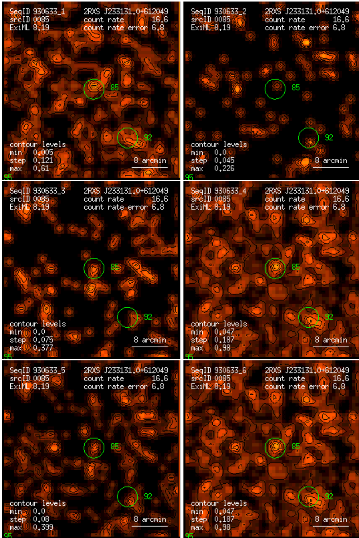
Figure 85: RASS 930633: detection 0085: band rate images, Gaussian filter: (1) PSPC channels 11 – 41, (2) 52 – 90, (3) 91 – 201, (4) 11 – 235, (5) 52 – 201, (6) 11 – 201. Broad band rates in counts/ks. Band rate contour levels in counts/ks/arcmin 2 .
