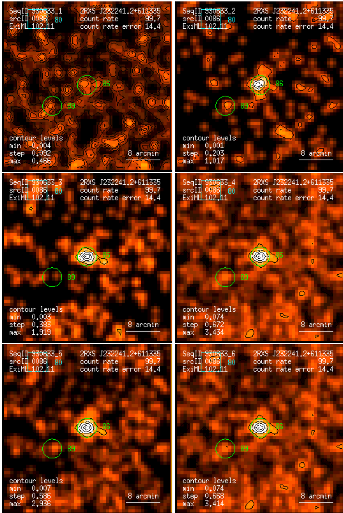
Figure 86: RASS 930633: detection 0086: band rate images, Gaussian filter: (1) PSPC channels 11 – 41, (2) 52 – 90, (3) 91 – 201, (4) 11 – 235, (5) 52 – 201, (6) 11 – 201. Broad band rates in counts/ks. Band rate contour levels in counts/ks/arcmin 2 .
