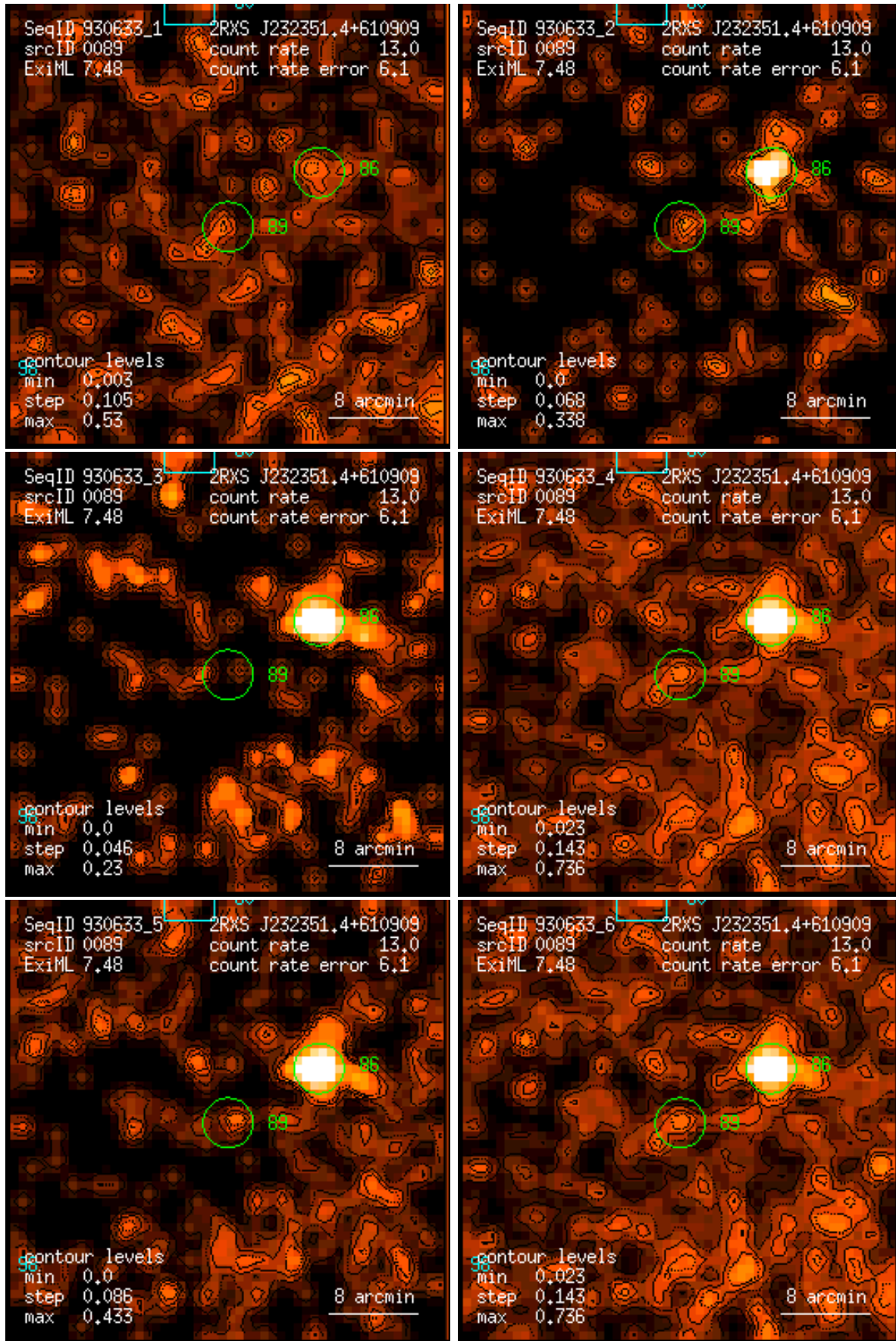
Figure 89: RASS 930633: detection 0089: band rate images, Gaussian filter: (1) PSPC channels 11 – 41, (2) 52 – 90, (3) 91 – 201, (4) 11 – 235, (5) 52 – 201, (6) 11 – 201. Broad band rates in counts/ks. Band rate contour levels in counts/ks/arcmin 2 .
