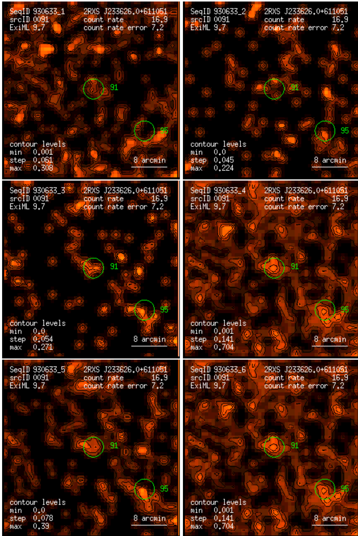
Figure 91: RASS 930633: detection 0091: band rate images, Gaussian filter: (1) PSPC channels 11 – 41, (2) 52 – 90, (3) 91 – 201, (4) 11 – 235, (5) 52 – 201, (6) 11 – 201. Broad band rates in counts/ks. Band rate contour levels in counts/ks/arcmin 2 .
