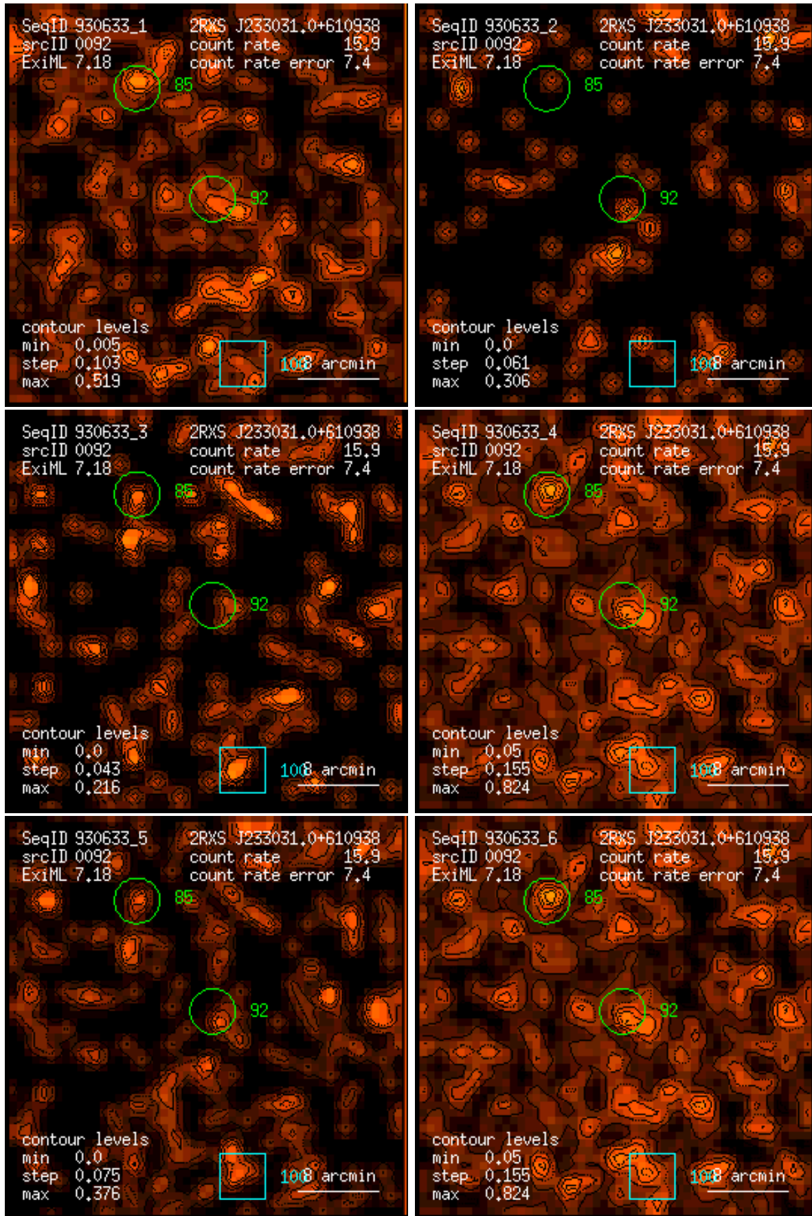
Figure 92: RASS 930633: detection 0092: band rate images, Gaussian filter: (1) PSPC channels 11 – 41, (2) 52 – 90, (3) 91 – 201, (4) 11 – 235, (5) 52 – 201, (6) 11 – 201. Broad band rates in counts/ks. Band rate contour levels in counts/ks/arcmin 2 .
