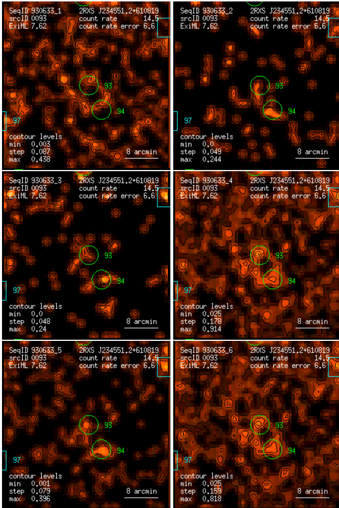
Figure 93: RASS 930633: detection 0093: band rate images, Gaussian filter: (1) PSPC channels 11 – 41, (2) 52 – 90, (3) 91 – 201, (4) 11 – 235, (5) 52 – 201, (6) 11 – 201. Broad band rates in counts/ks. Band rate contour levels in counts/ks/arcmin 2 .
