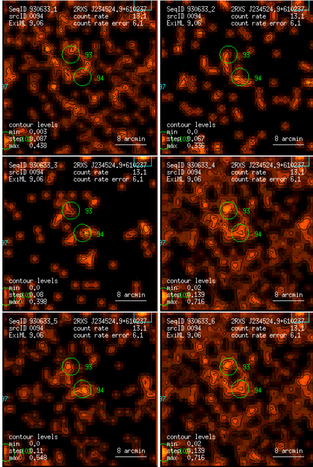
Figure 94: RASS 930633: detection 0094: band rate images, Gaussian filter: (1) PSPC channels 11 – 41, (2) 52 – 90, (3) 91 – 201, (4) 11 – 235, (5) 52 – 201, (6) 11 – 201. Broad band rates in counts/ks. Band rate contour levels in counts/ks/arcmin 2 .
