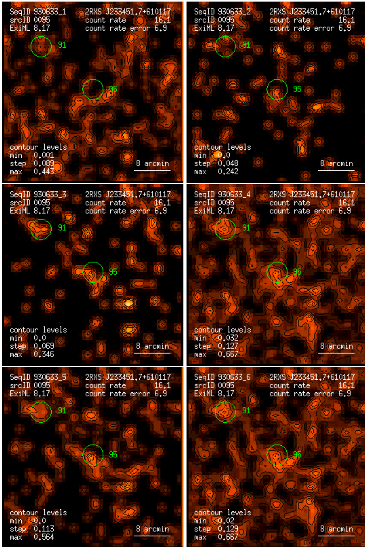
Figure 95: RASS 930633: detection 0095: band rate images, Gaussian filter: (1) PSPC channels 11 – 41, (2) 52 – 90, (3) 91 – 201, (4) 11 – 235, (5) 52 – 201, (6) 11 – 201. Broad band rates in counts/ks. Band rate contour levels in counts/ks/arcmin 2 .
