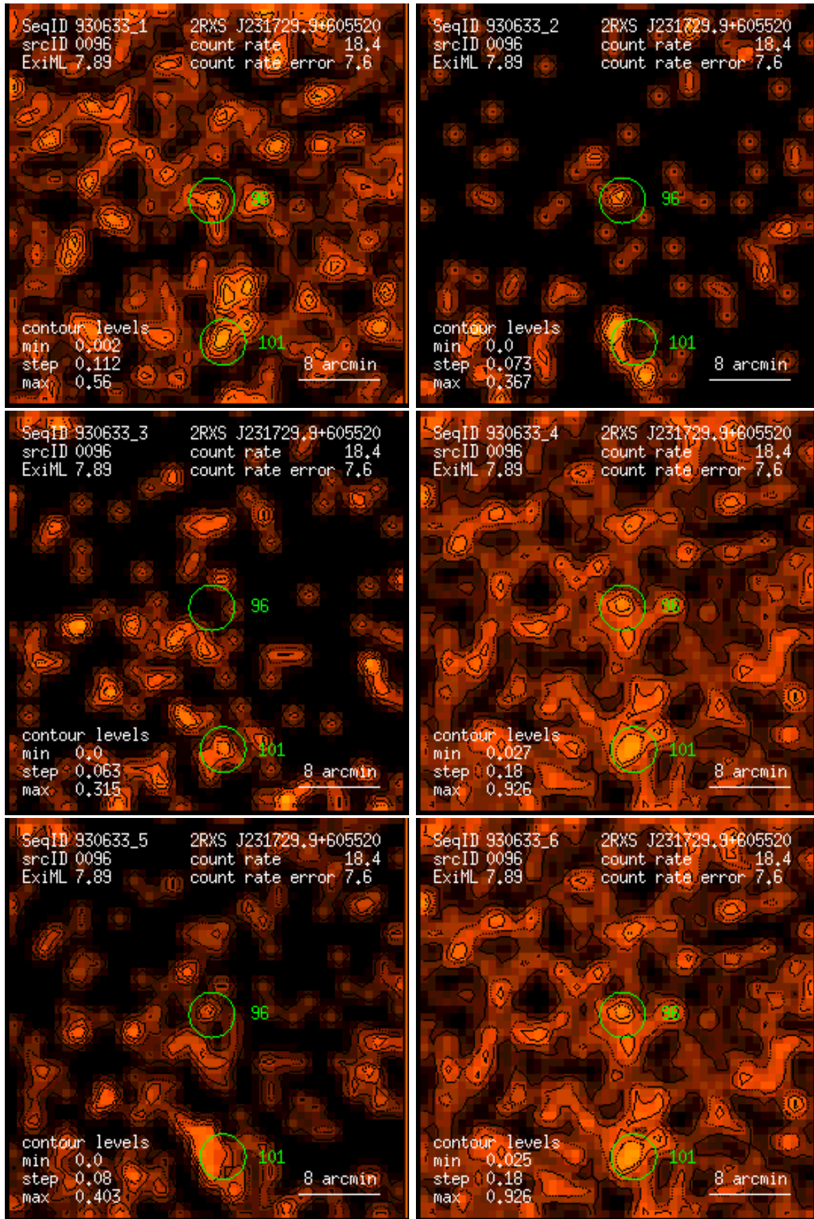
Figure 96: RASS 930633: detection 0096: band rate images, Gaussian filter: (1) PSPC channels 11 – 41, (2) 52 – 90, (3) 91 – 201, (4) 11 – 235, (5) 52 – 201, (6) 11 – 201. Broad band rates in counts/ks. Band rate contour levels in counts/ks/arcmin 2 .
