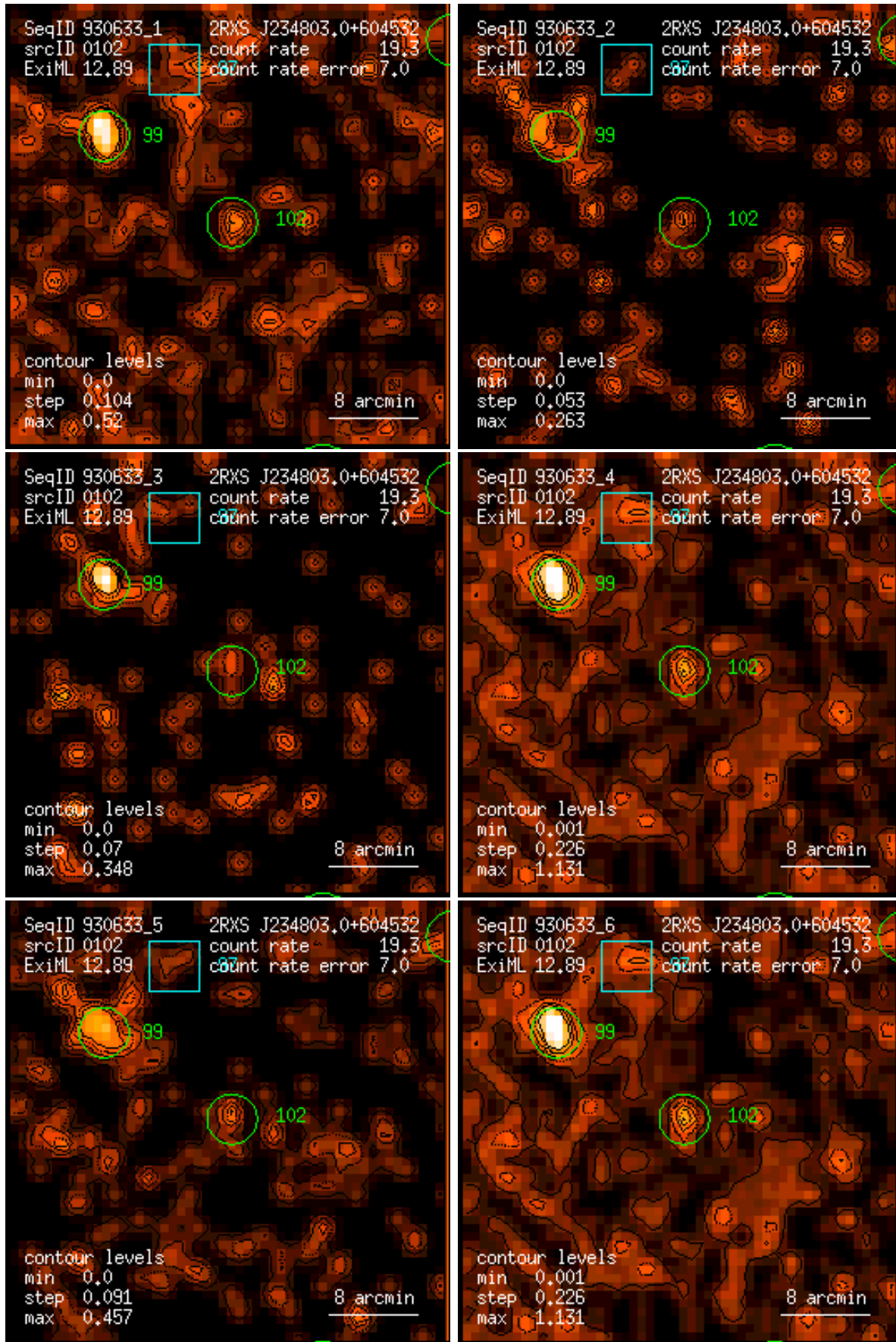
Figure 102: RASS 930633: detection 0102: band rate images, Gaussian filter: (1) PSPC channels 11 – 41, (2) 52 – 90, (3) 91 – 201, (4) 11 – 235, (5) 52 – 201, (6) 11 – 201. Broad band rates in counts/ks. Band rate contour levels in counts/ks/arcmin 2 .
