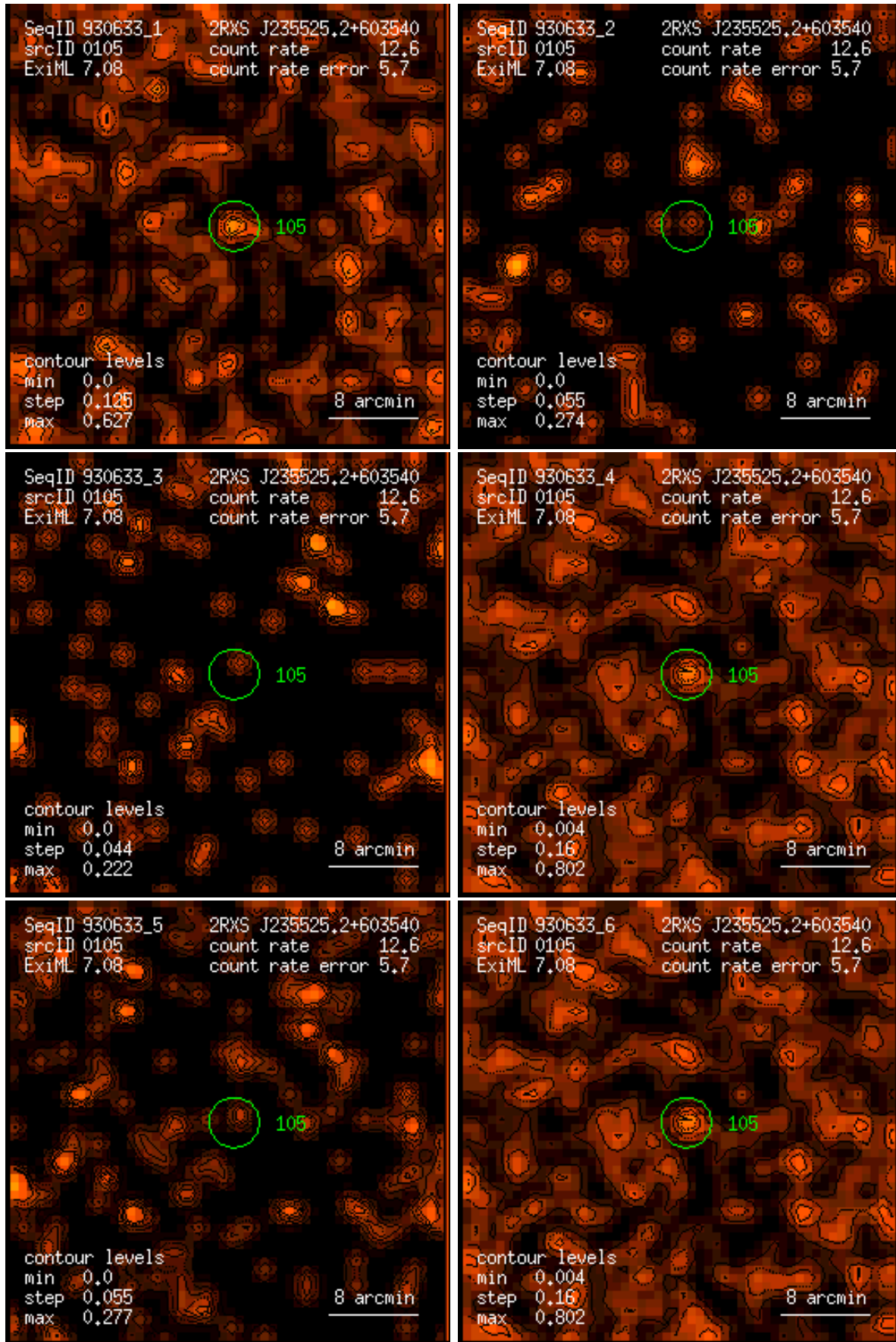
Figure 105: RASS 930633: detection 0105: band rate images, Gaussian filter: (1) PSPC channels 11 – 41, (2) 52 – 90, (3) 91 – 201, (4) 11 – 235, (5) 52 – 201, (6) 11 – 201. Broad band rates in counts/ks. Band rate contour levels in counts/ks/arcmin 2 .
