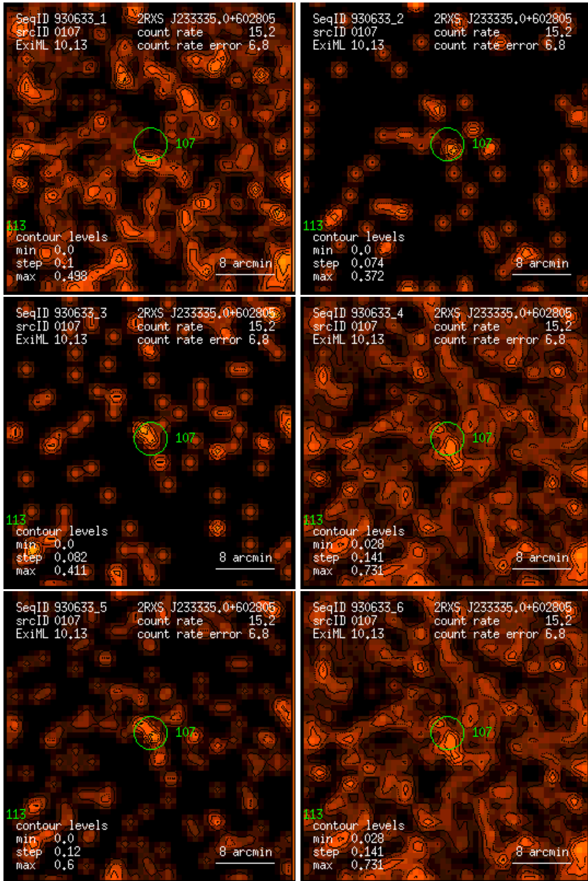
Figure 107: RASS 930633: detection 0107: band rate images, Gaussian filter: (1) PSPC channels 11 – 41, (2) 52 – 90, (3) 91 – 201, (4) 11 – 235, (5) 52 – 201, (6) 11 – 201. Broad band rates in counts/ks. Band rate contour levels in counts/ks/arcmin 2 .
