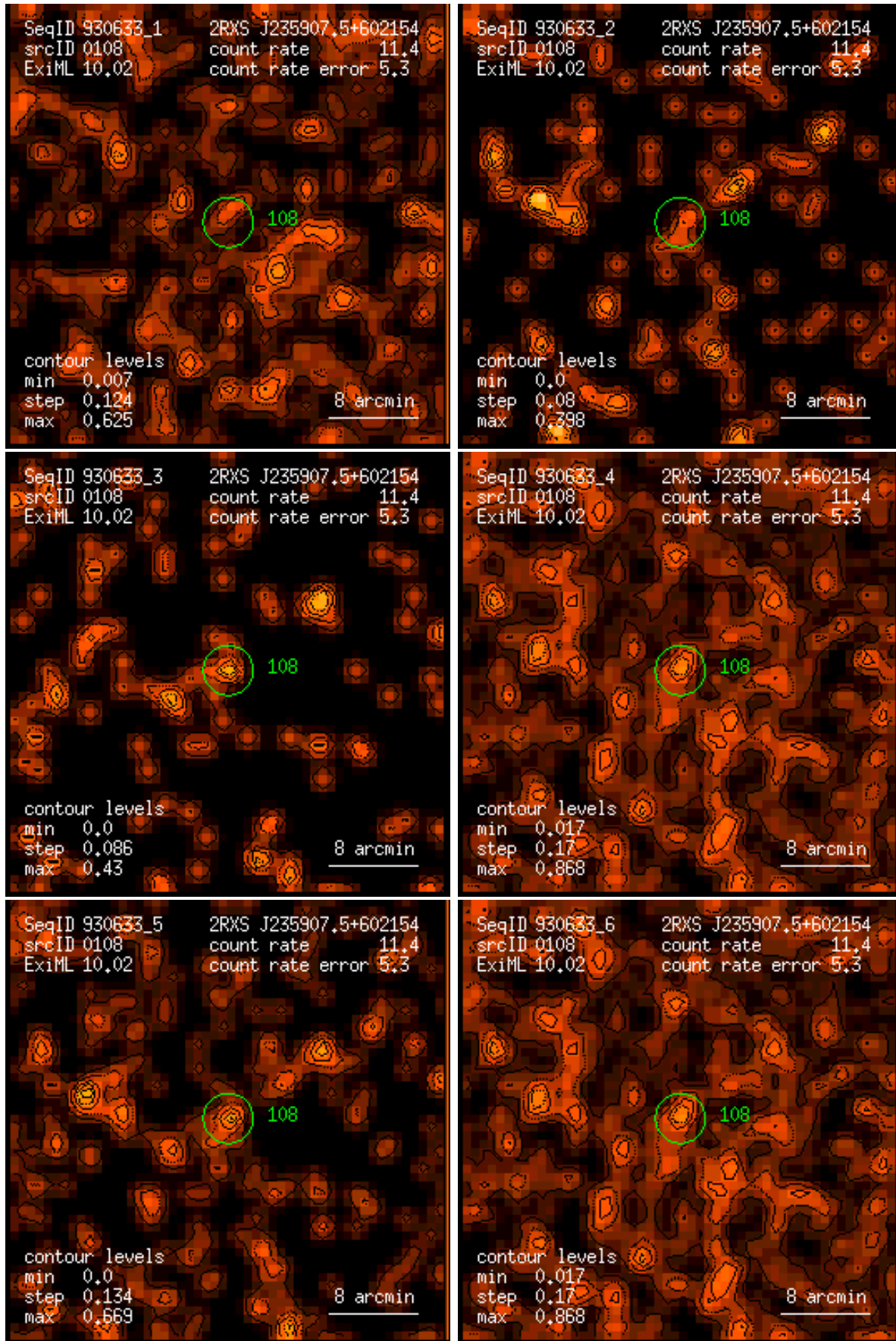
Figure 108: RASS 930633: detection 0108: band rate images, Gaussian filter: (1) PSPC channels 11 – 41, (2) 52 – 90, (3) 91 – 201, (4) 11 – 235, (5) 52 – 201, (6) 11 – 201. Broad band rates in counts/ks. Band rate contour levels in counts/ks/arcmin 2 .
