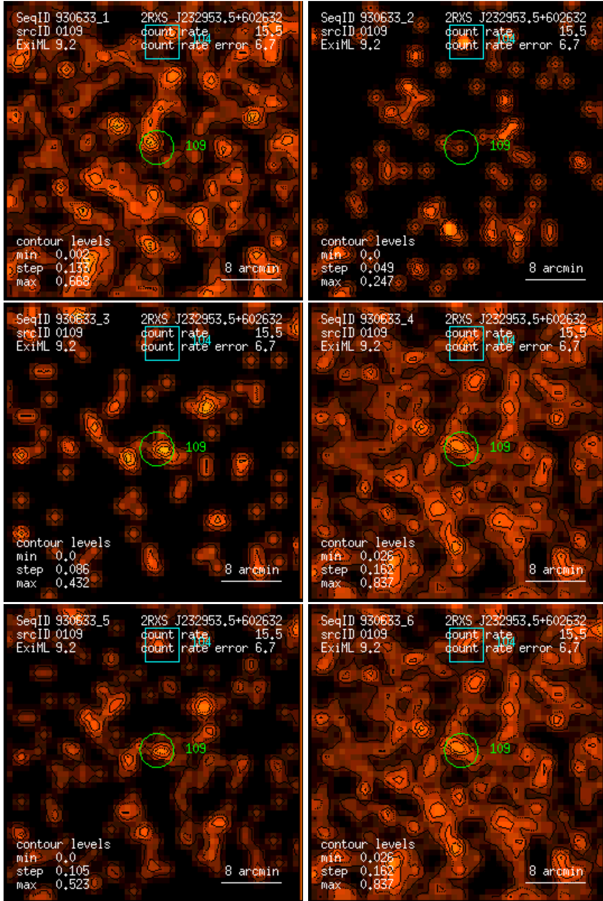
Figure 109: RASS 930633: detection 0109: band rate images, Gaussian filter: (1) PSPC channels 11 – 41, (2) 52 – 90, (3) 91 – 201, (4) 11 – 235, (5) 52 – 201, (6) 11 – 201. Broad band rates in counts/ks. Band rate contour levels in counts/ks/arcmin 2 .
