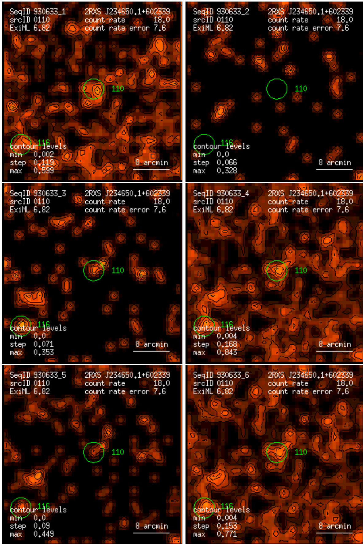
Figure 110: RASS 930633: detection 0110: band rate images, Gaussian filter: (1) PSPC channels 11 – 41, (2) 52 – 90, (3) 91 – 201, (4) 11 – 235, (5) 52 – 201, (6) 11 – 201. Broad band rates in counts/ks. Band rate contour levels in counts/ks/arcmin 2 .
