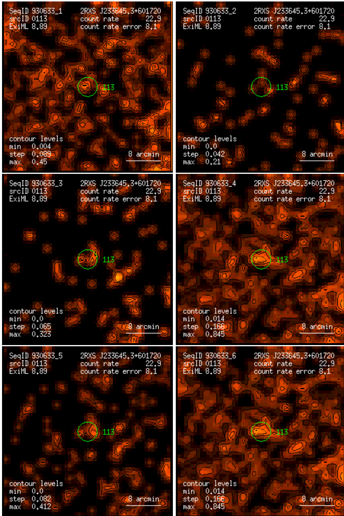
Figure 113: RASS 930633: detection 0113: band rate images, Gaussian filter: (1) PSPC channels 11 – 41, (2) 52 – 90, (3) 91 – 201, (4) 11 – 235, (5) 52 – 201, (6) 11 – 201. Broad band rates in counts/ks. Band rate contour levels in counts/ks/arcmin 2 .
